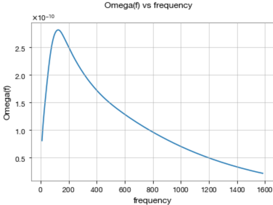
Figure 7: For the above plot, we have taken a minimum black hole mass of 5 solar masses and a maximum black hole mass of 100 solar masses, a minimum neutron star mass of 1.5 solar masses
