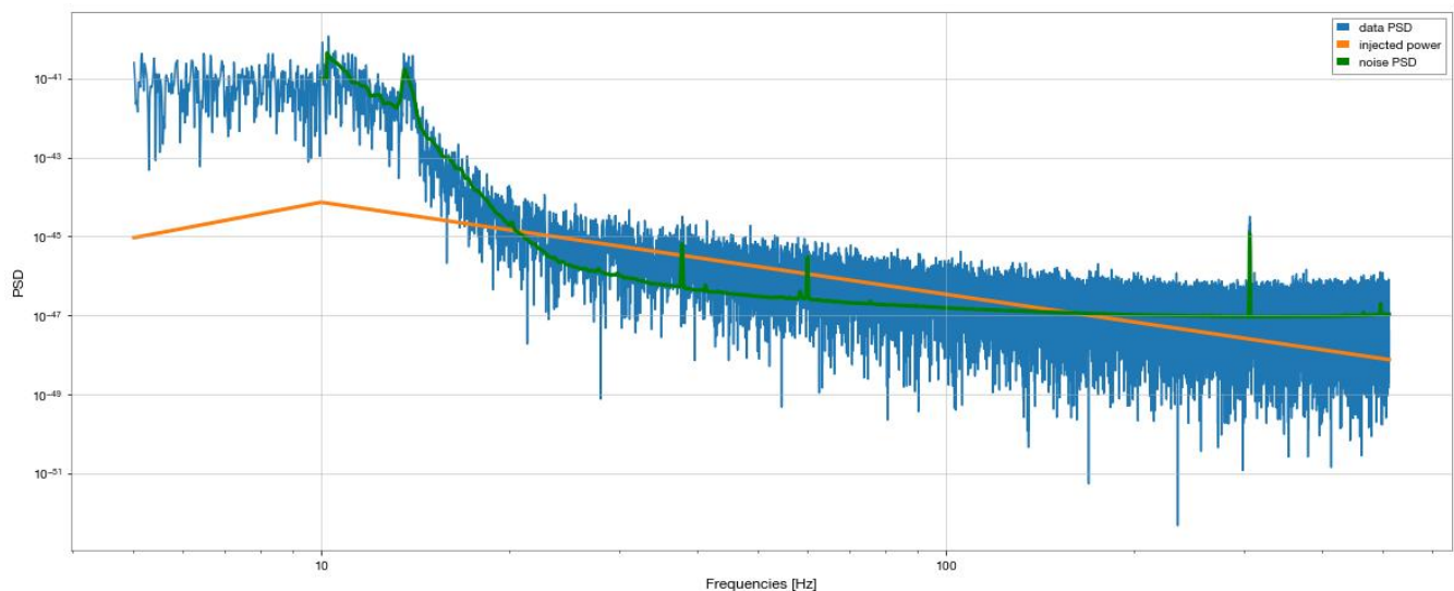
Figure 3: Visualizing the data PSD (shown in blue), an injected curve representing the broken power law (shown in orange), and the original noise curve (shown in green). This graph identifies the final result after injecting a broken power law into the LIGO noise data, and is emblematic of the PSD signature, which we may expect with a SGWB within noise data. Here,
