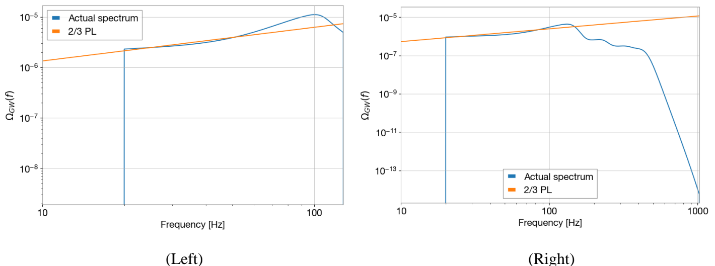
Figure 8: \Omega_{GW}(f) over a frequency range compared to a power law of 2/3 [18]. The priors that we specify are the average ratio of the masses in CBCs, the average masses themselves, luminosity distance, and a host of other variables [18]. If we set all other variables to 0, set luminosity distance to a power law function with a minimum of 100 Mpc to 1000 Mpc, we can get the above Figure 8 (left and right) through an average mass ratio of 1.0, and setting both priors for mass 1 and mass 2 to uniform distributions with a minimum of 1.5 and a maximum of 100 solar masses [18]. Note that 10 injections were used to create Figure 8 (left and right) above, which is why the graph of \Omega_{GW}(f) begins to become more stochastic at higher frequencies [18].
