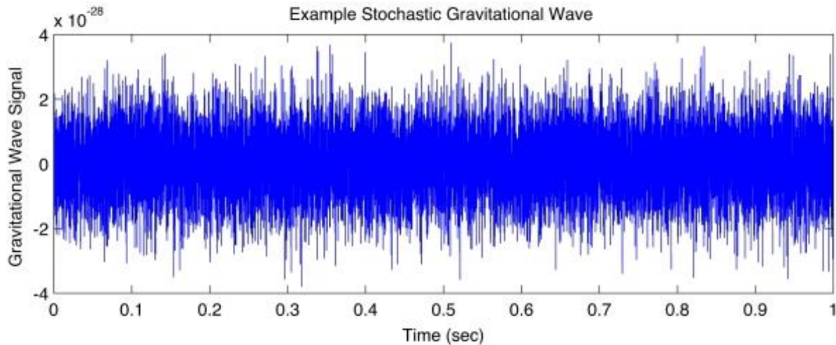
Figure 2: An example signal from a stochastic GW source. The signal is roughly uniform in amplitude and frequency in time, and is very faint [10].
