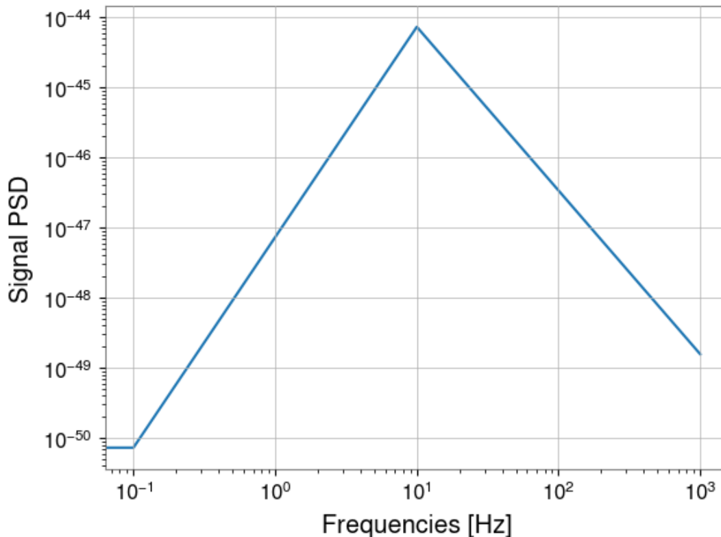
Figure 4: A closer look at an example of broken power law representing a signal PSD from a hypothetical stochastic signal over a frequency distribution that we may expect [12].
