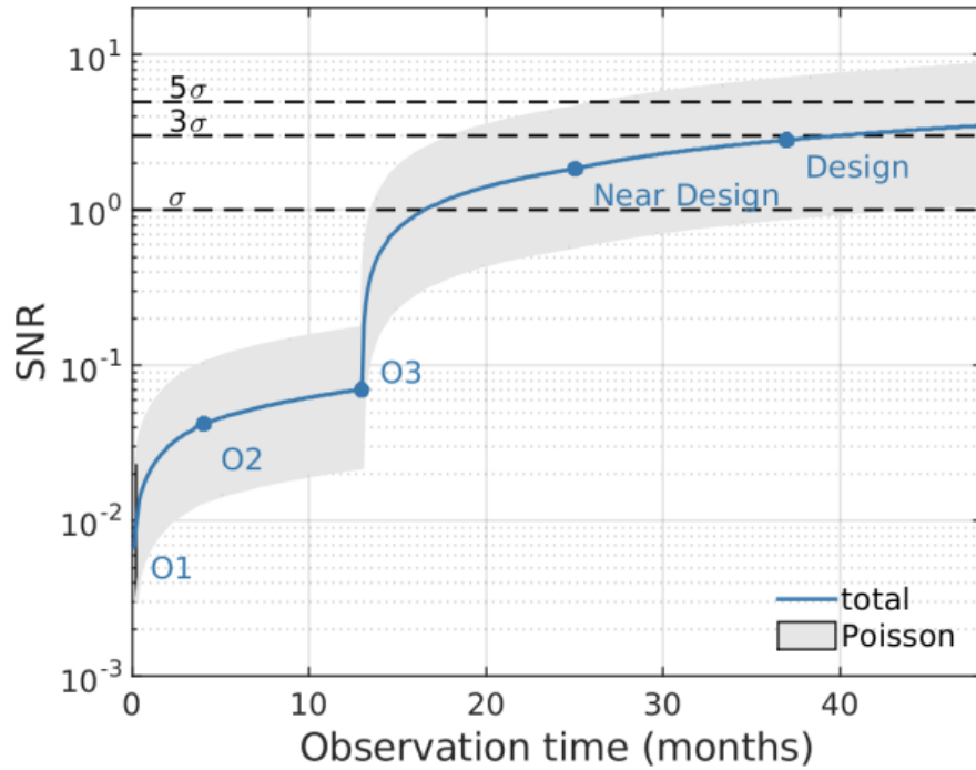
Figure 5: The image above shows the improvements in detector SNR [6]. As SNR will increase, the level of the SGWB will also be reached by the LVK network [6]. Therefore, overall, given the energy densities that can be measurable by upcoming detectors is also taken into account, we can understand that we should be able to detect the SGWB within a few years. The result of this research project will, hence, contribute to further constraining and understanding of the methodologies used to construct predictions of the SGWB, as well as decode the range of possible predictions from simulation [6].
