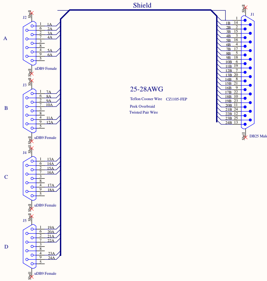
J2, J3, J4, J5 - 9 Pin micro-dsub Backshell
