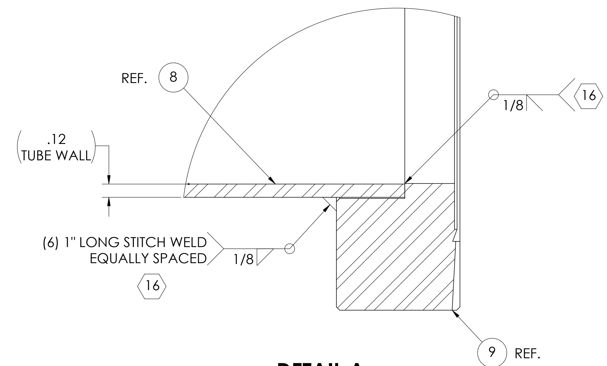
DETAIL A SCALE 2:1 TYPICAL
