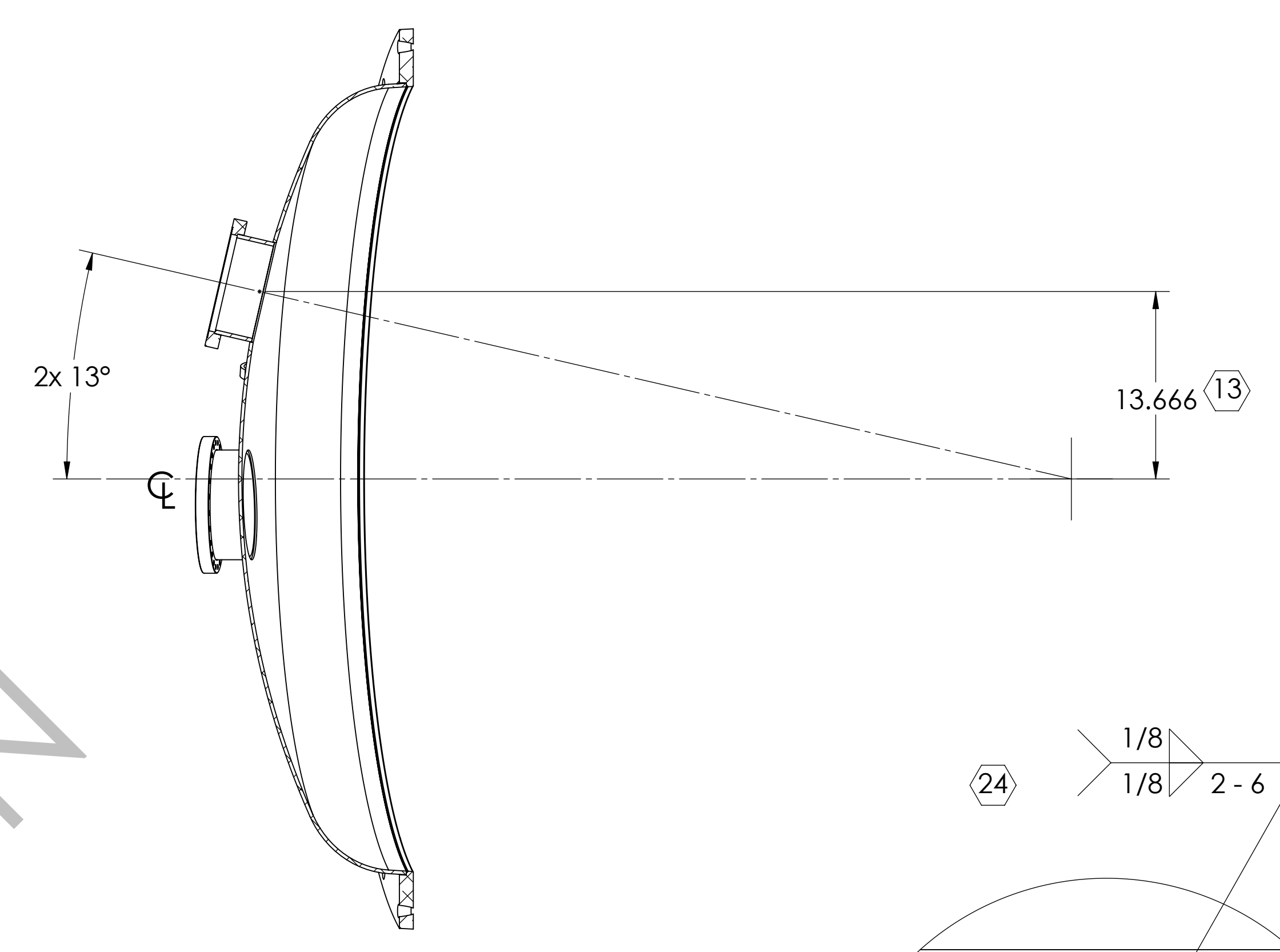
SECTION B-B (ROTATED 80.0° CW)
