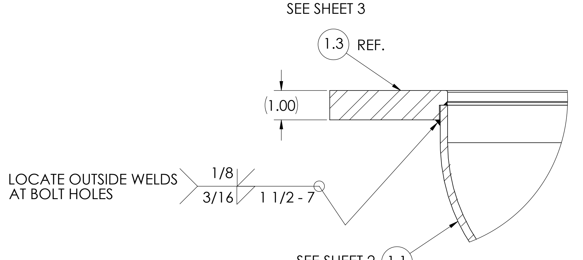
DETAIL C SCALE 1 : 2
