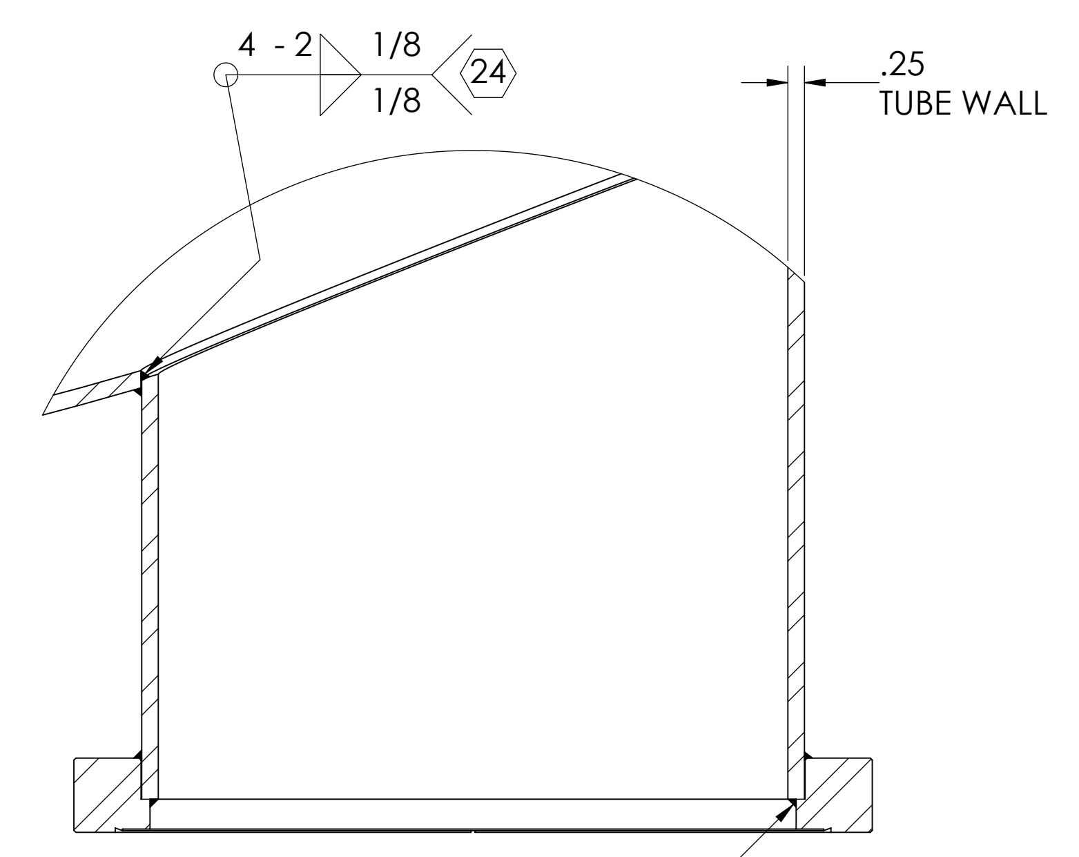
DETAIL K SCALE 1 : 2
