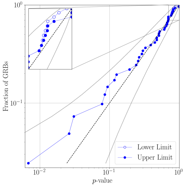
Figure 1. The cumulative distribution of event p -values for the NS binary search in O2. If the search reports no trigger in the on-source we plot an upper limit on the p -value of 1, and a lower limit equal to the number of off-source trials that contained no trigger. The dashed line indicates the expected distribution of p -values under the no-signal hypothesis, with the corresponding 2\sigma envelope marked by dotted lines.
