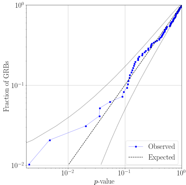
Figure 3. Cumulative distribution of p -values from the unmodeled search for transient GWs associated with 97 GRBs. The dashed line represents the expected distribution under the no-signal hypothesis, with dotted lines indicating a 2\sigma deviation from this distribution. These results are consistent with the no-signal hypothesis, and have a combined p -value of 0.75 as calculated by a weighted binomial test (Abadie et al. 2012b).
