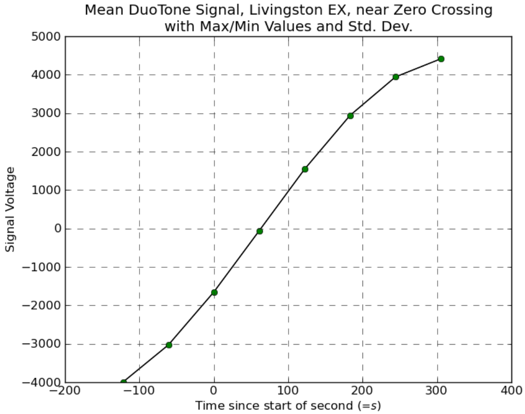
Figure 8: Zero crossing region of the second-to-second average of the DuoTone witness signals around the second edge at Livingston EX for the hour surrounding the GW151226 event candidate. The line through the data points guide the eye to help visualize the zero crossing. Please note that the errors on each point are so small that they are covered by the circular symbol.
