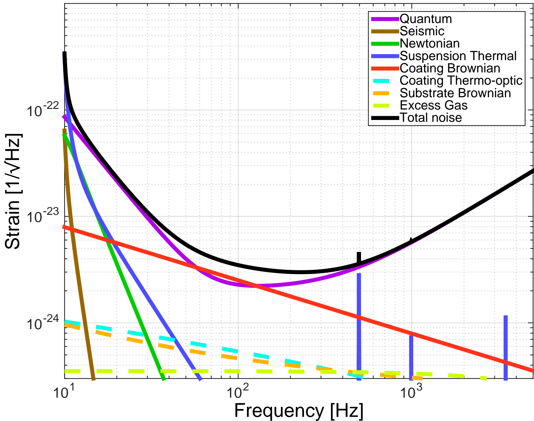
aLIGO Noise Curve: P_{in} = 125.0 W
