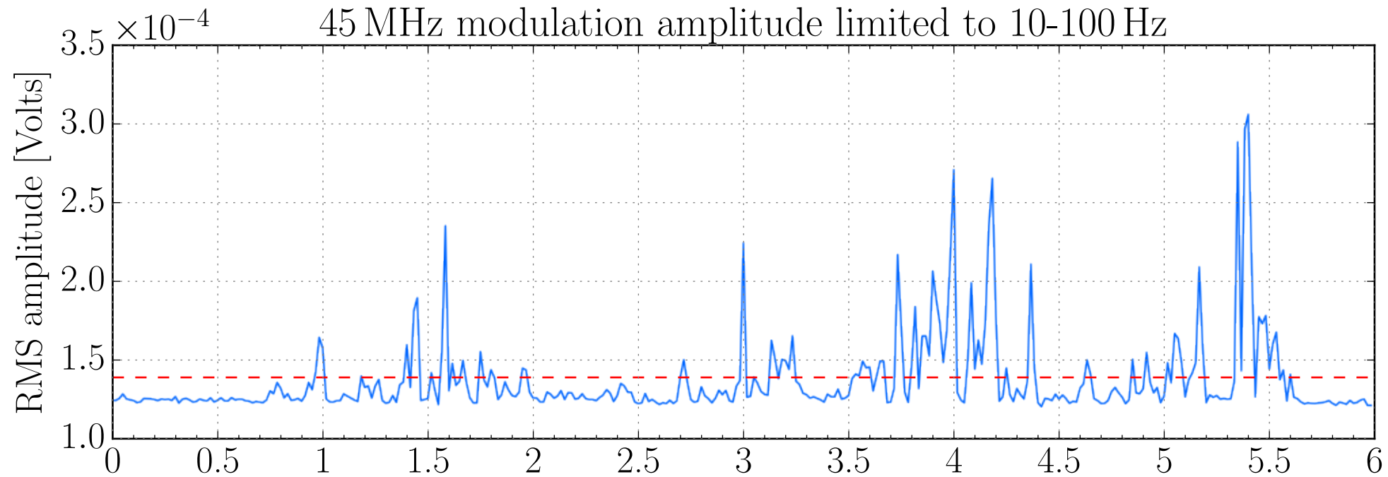
Noise transients in h(t)
