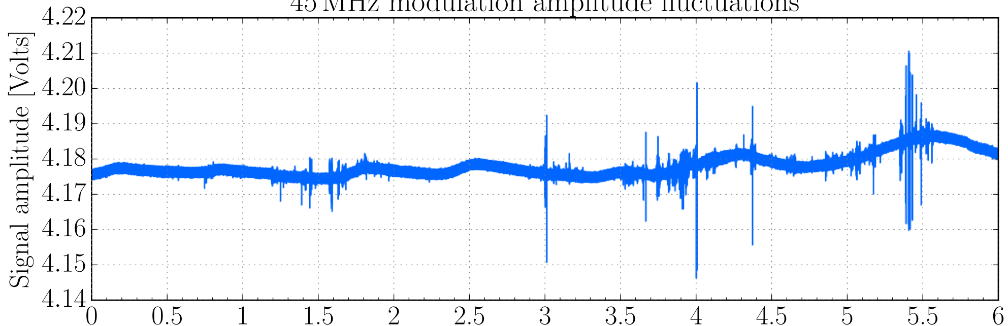
45 MHz modulation amplitude limited to 10-100 Hz
