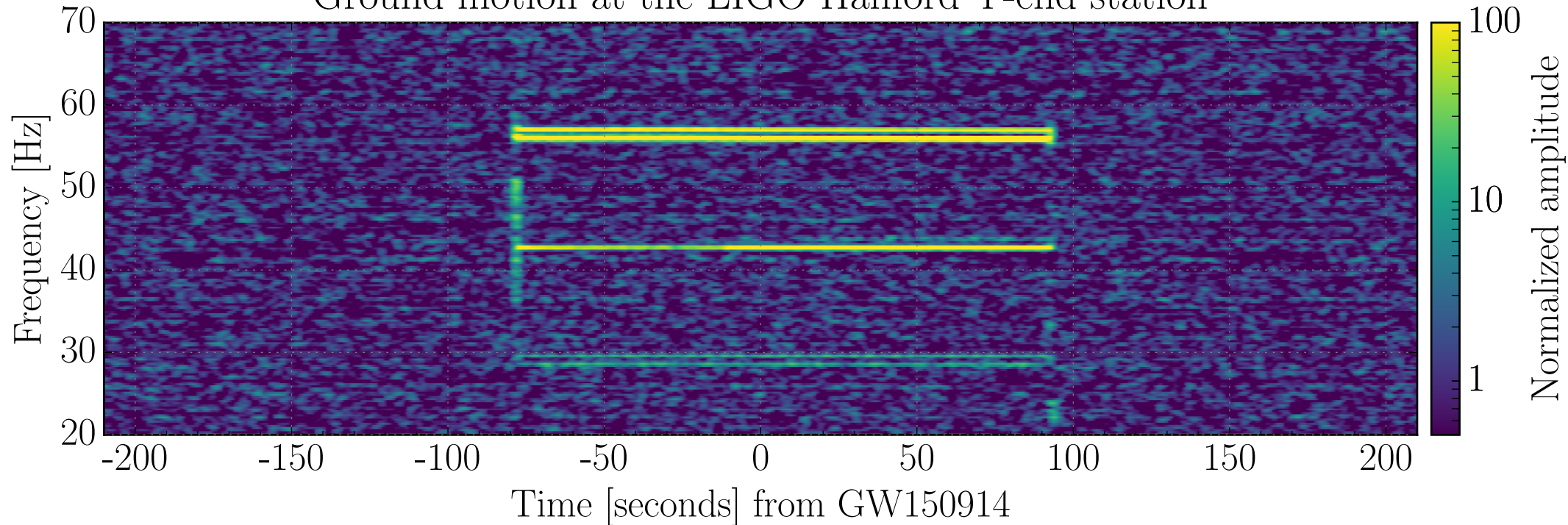
Ground motion at the LIGO Hanford Y-end station
