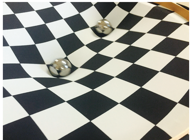
Figure 4: Merging Black Holes
