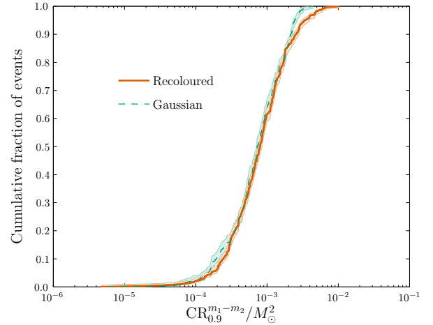
Figure 17. Cumulative fractions of events with m_1-m_2 90% credible regions smaller than the abscissa value. Results using recoloured noise are indicated by a solid line and the results using Gaussian noise (Singer et al. 2014) are indicated by a dashed line. The 68% confidence intervals are denoted by the shaded areas. These results show the typical posterior width using non-spinning waveforms, the failure to include the mass-spin degeneracy means that these posteriors are too narrow.
