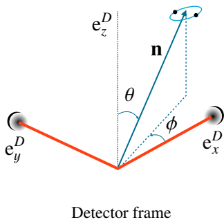
Figure 1.2: Coordinate systems for describing gravitational waves. We define three convenient coordinate systems for describing gravitational waves and the related angular parameters which transform from one frame to another. Figure courtesy of P. Ajith.
