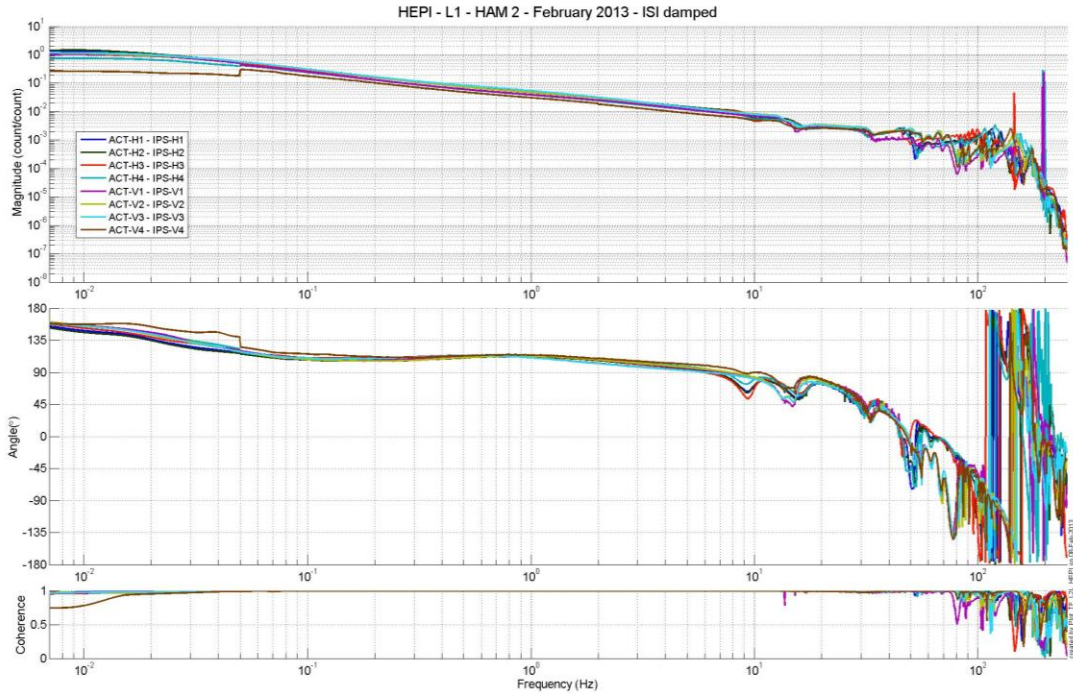
Figure 23: L1 HAM 4 HEPI Act to IPS Transfer Functions
