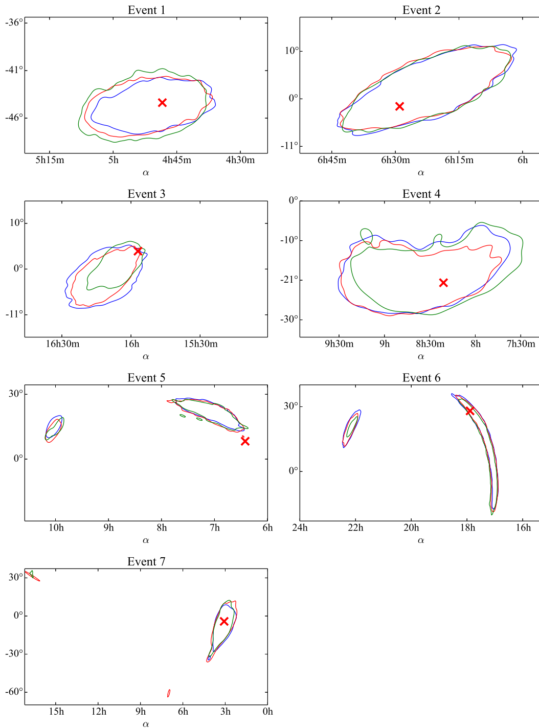
Figure 10. 95% credible regions for the sky position of all seven events, using the EOBNRv2 (blue), \text{PhenomB}_{\chi=0} (red), and \text{PhenomB} (green) models. Despite the substantial differences between these models, their sky localization ability is very consistent.
