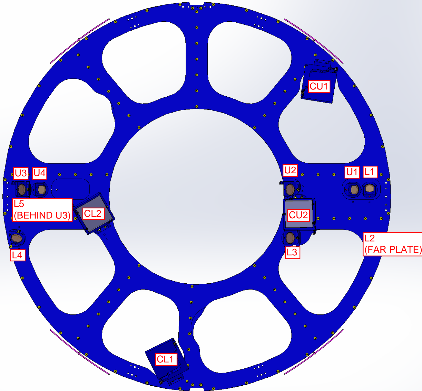
-02 PERISCOPE (X-ARM)
