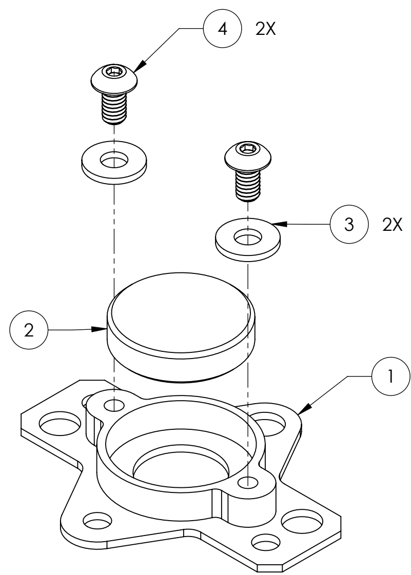
ISO VIEW
