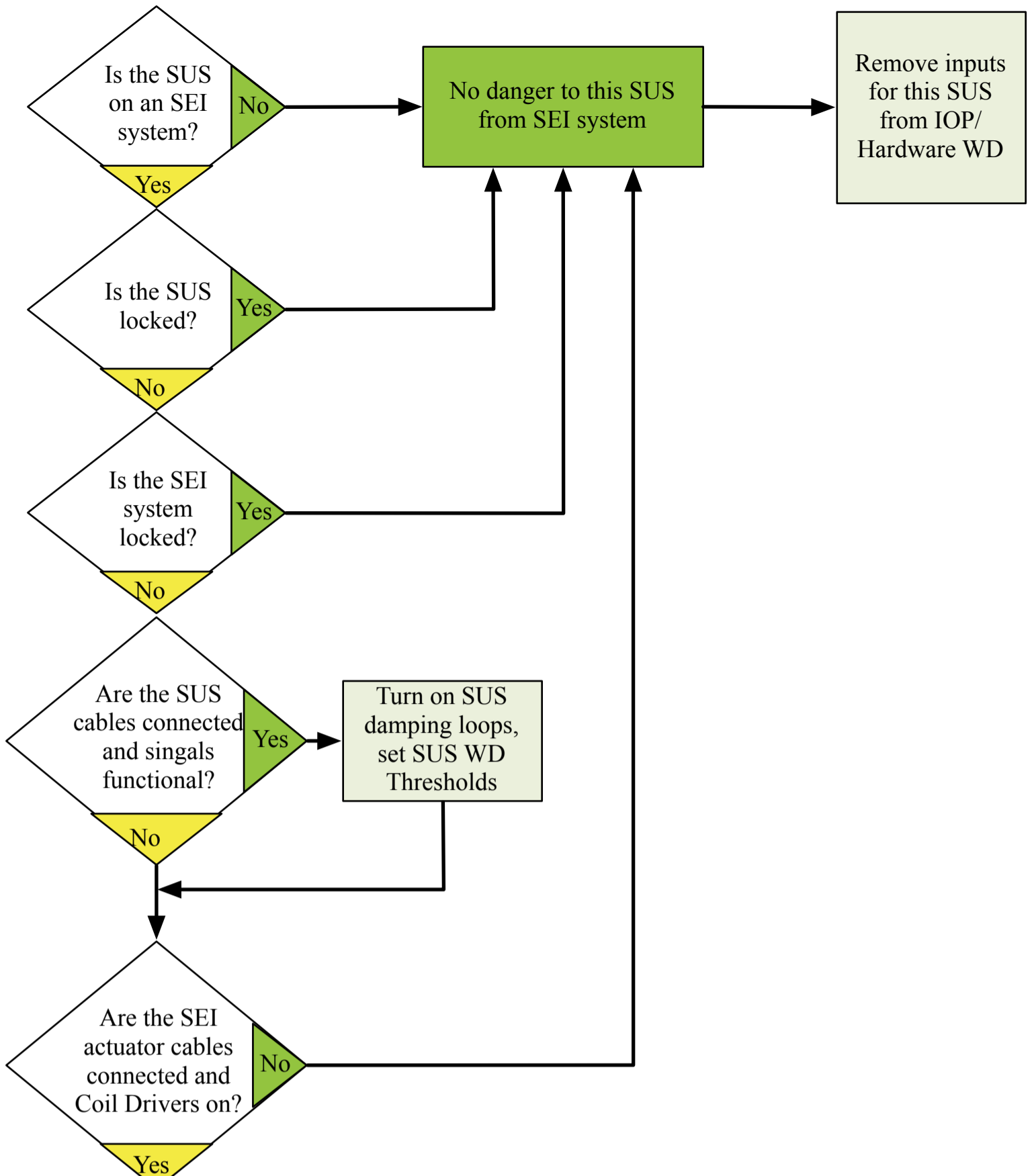
IOP/Hardware Watchdog Need Assessment Flow Chart T1200482-v2 J. Kissel
