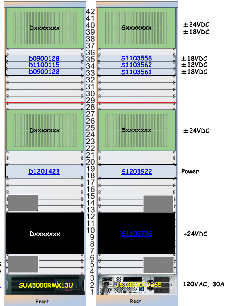
PSL Rack 1 Layout ( D1201120 ) ( S1202978 )
