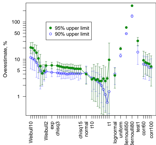
FIG. 5. Average overestimate of upper limit by the additive universal statistic as compared to the value predicted by analytical formula for the corresponding distributions. The overestimate is less than 5% for Gaussian data, and we expect any practical measurement to perform worse than the ideal case. The error bars show region containing 90% of upper limits from different noise realizations. The upper limits were computed using f_c (see figure 2) with N = 501 points of data for different noise distributions described in the text. The points on the graph were obtained by averaging 100 independent measurements, each of which consisted of finding the maximum among L = 100 upper limits to simulate maximization across a set of templates. (color online)
