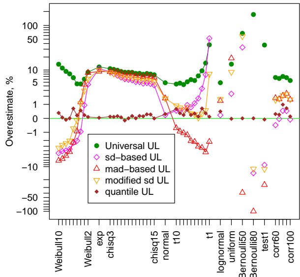
FIG. 9. Average overestimate of upper limit by various methods as compared to the value predicted by analytical formula for the corresponding distributions. This plots shows 95% confidence level upper limit for batch size L = 1 as described in text. (color online)
