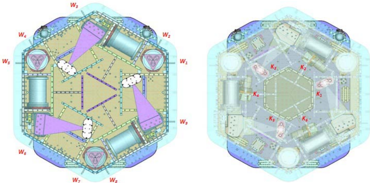
Figure – Keel Masses and Wall masses location
