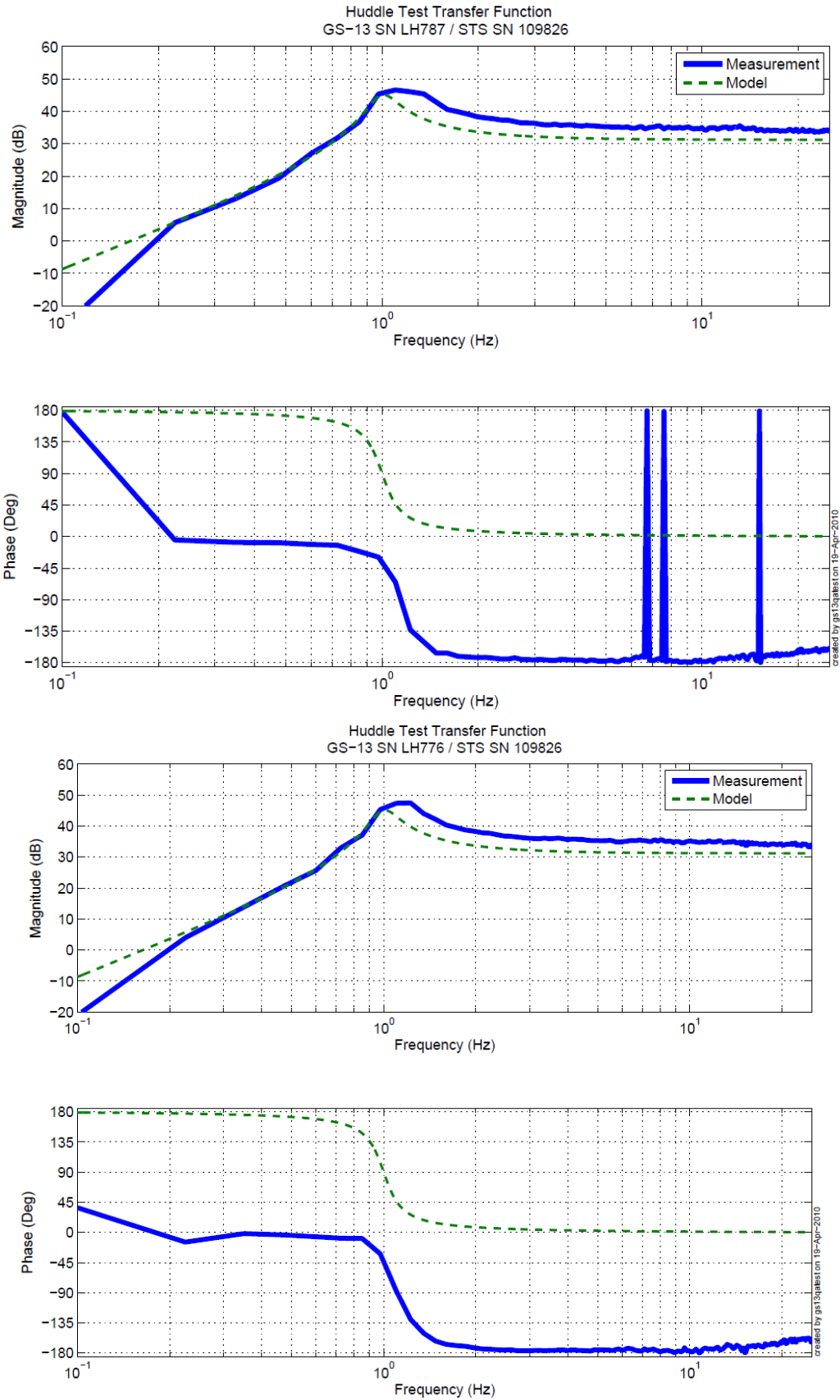
Figure - Huddle testing of Horiz GS-13 809, 787 and 706 after aLIGO modifications
