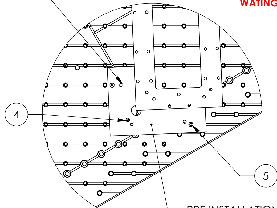
DETAIL A SCALE 1 : 6 PRE INSTALLATION PLATE
