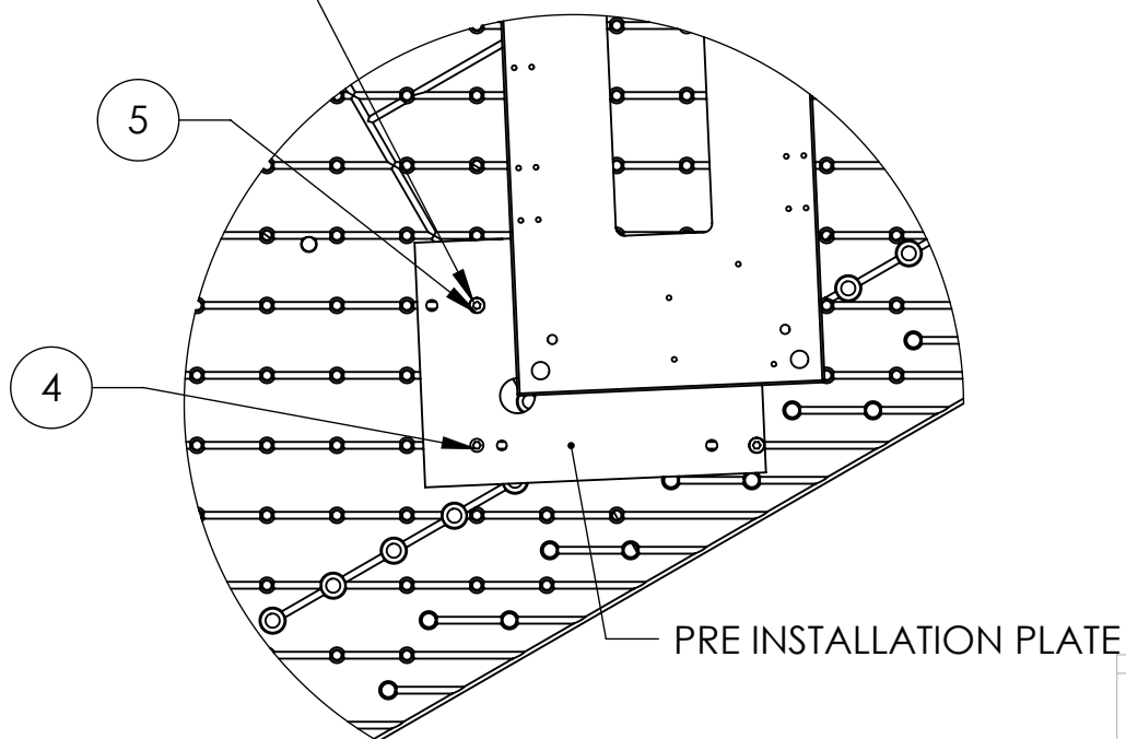
DETAIL A SCALE 1 : 6
