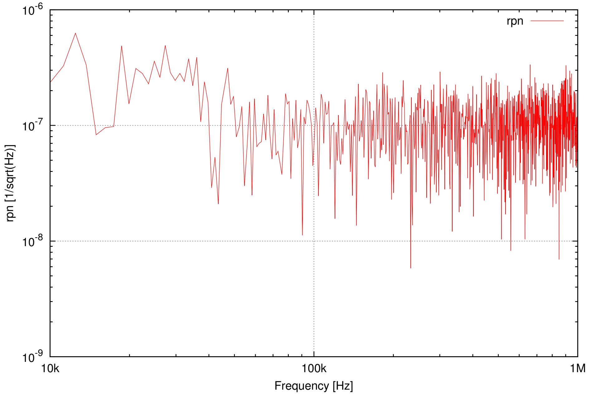
35W amplifier relative power noise at high frequencies
