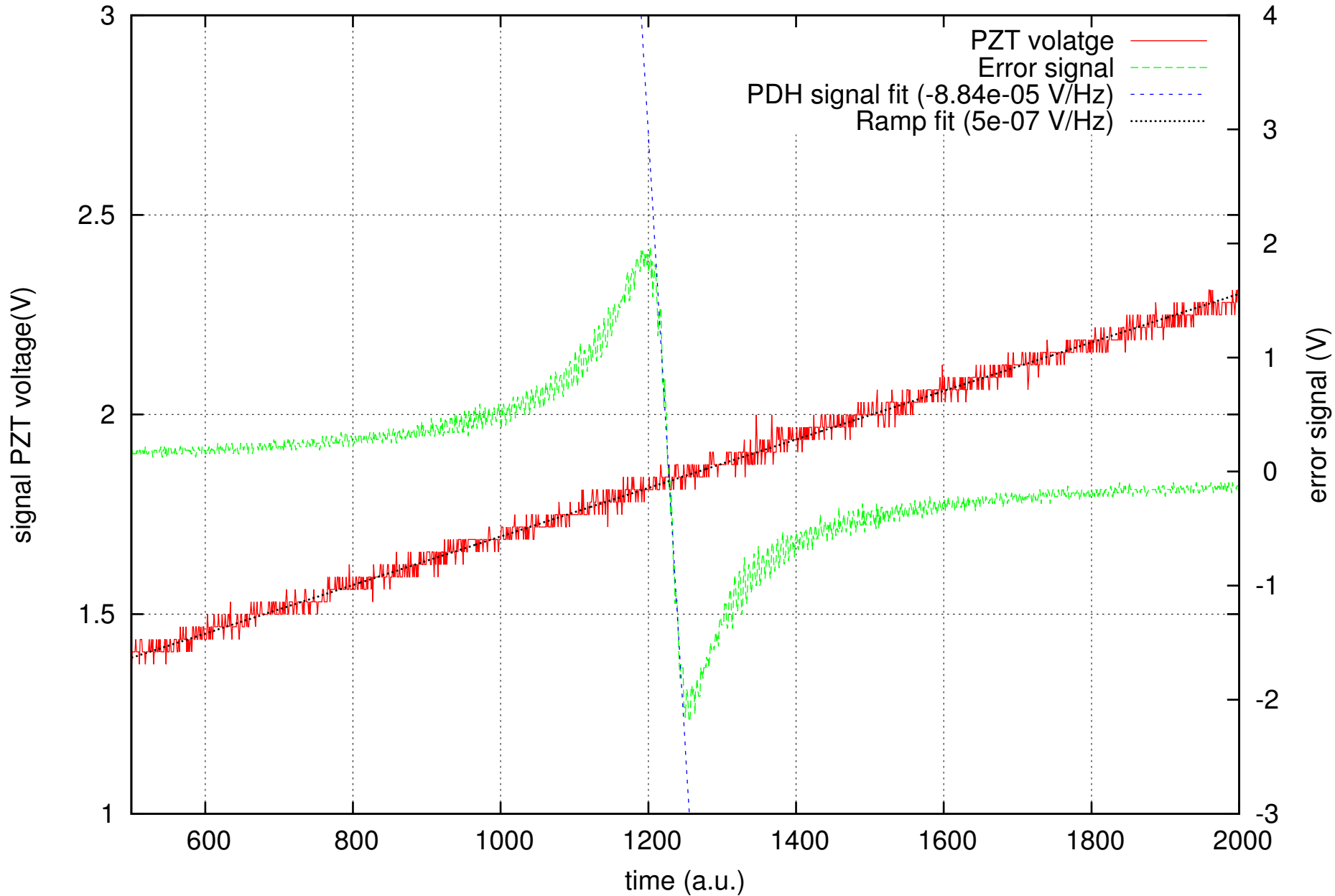
Error signal of FSS
