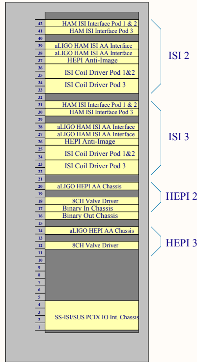
HAMs 2&3 L1-SEI-C2
