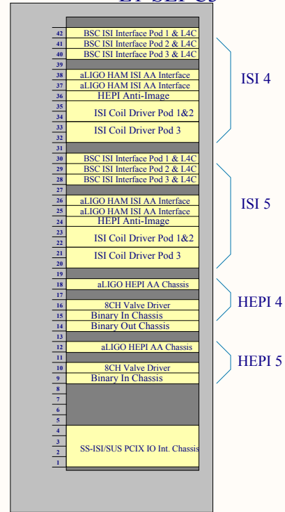
HAMs 4&5 L1-SEI-C3
