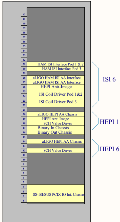
HAMs 1&6 L1-SEI-C1
