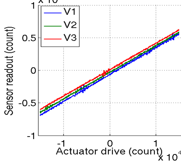
Figure 5 - Linearity Test
