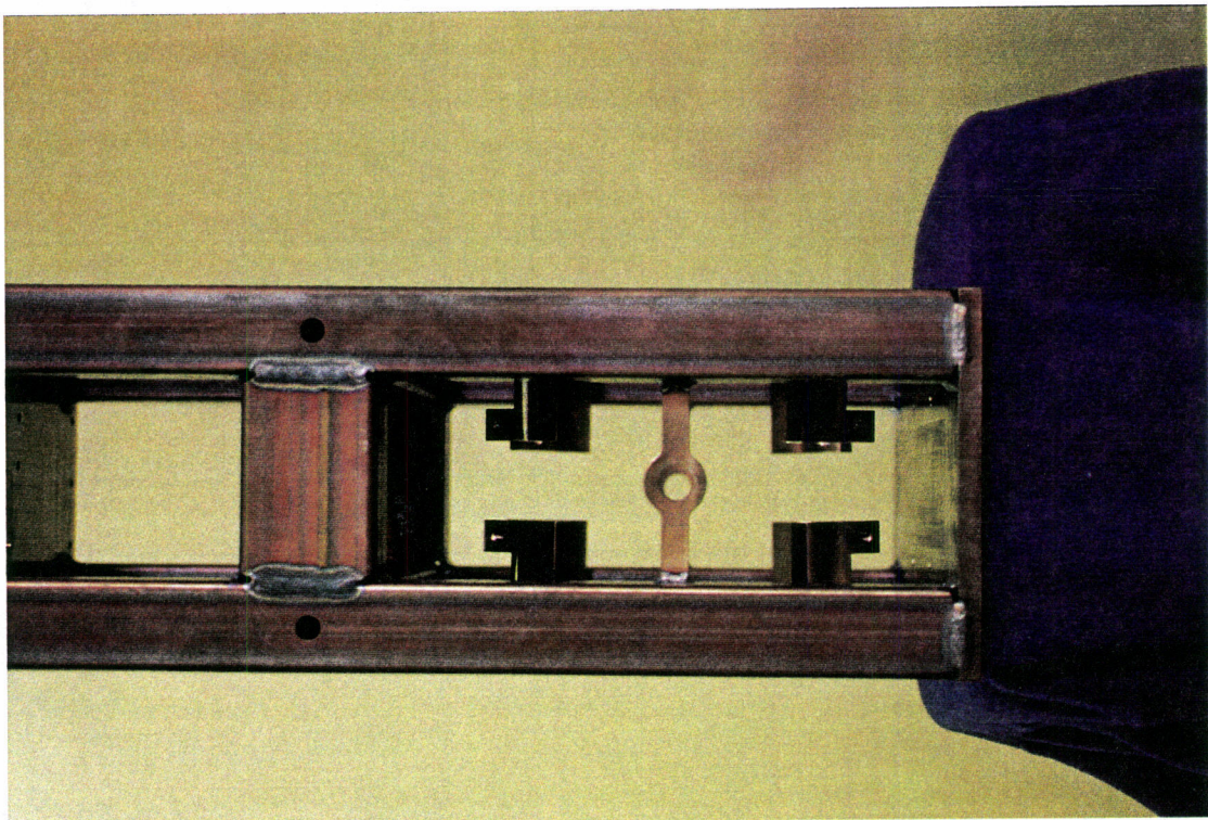
LIGO-G960133-08-D LOS Prototype, Incomplete Side View
