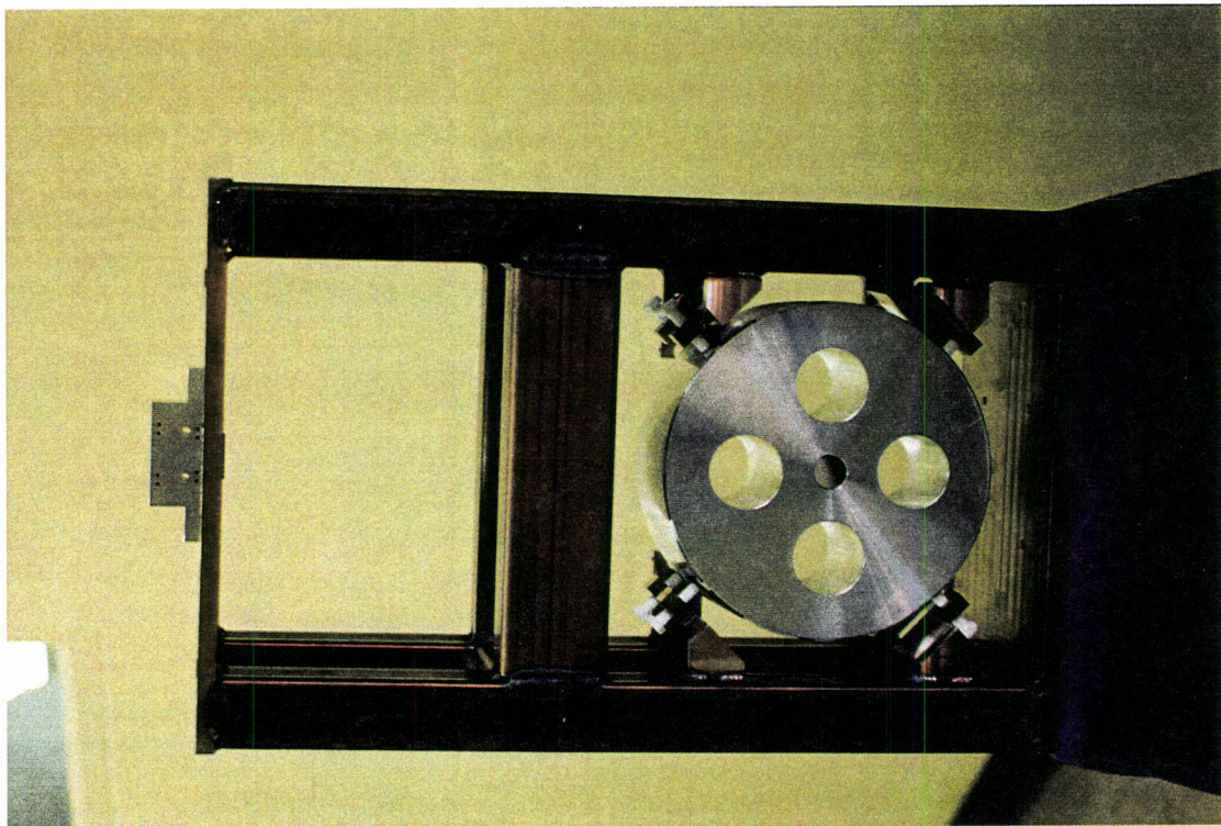
LIGO-G960133-04-D LOS Prototype, Incomplete Front View with Suspension Block Aluminum Test Mass, Side Safety Stops
