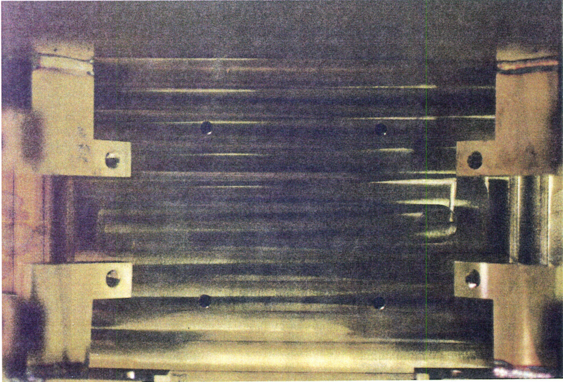
LIGO-G960133-03-D LOS Prototype, Incomplete Top View Through Hole in Top Plate
