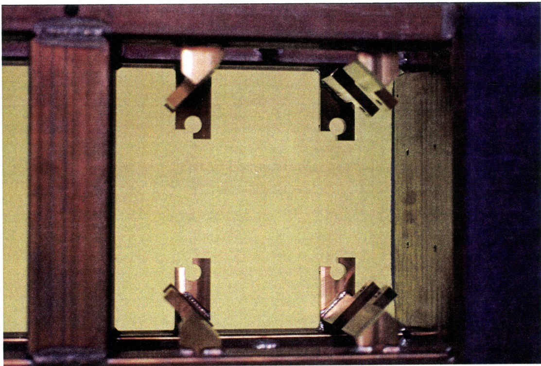
LIGO-G960133-12-D LOS Prototype, Incomplete Bottom of Front View
