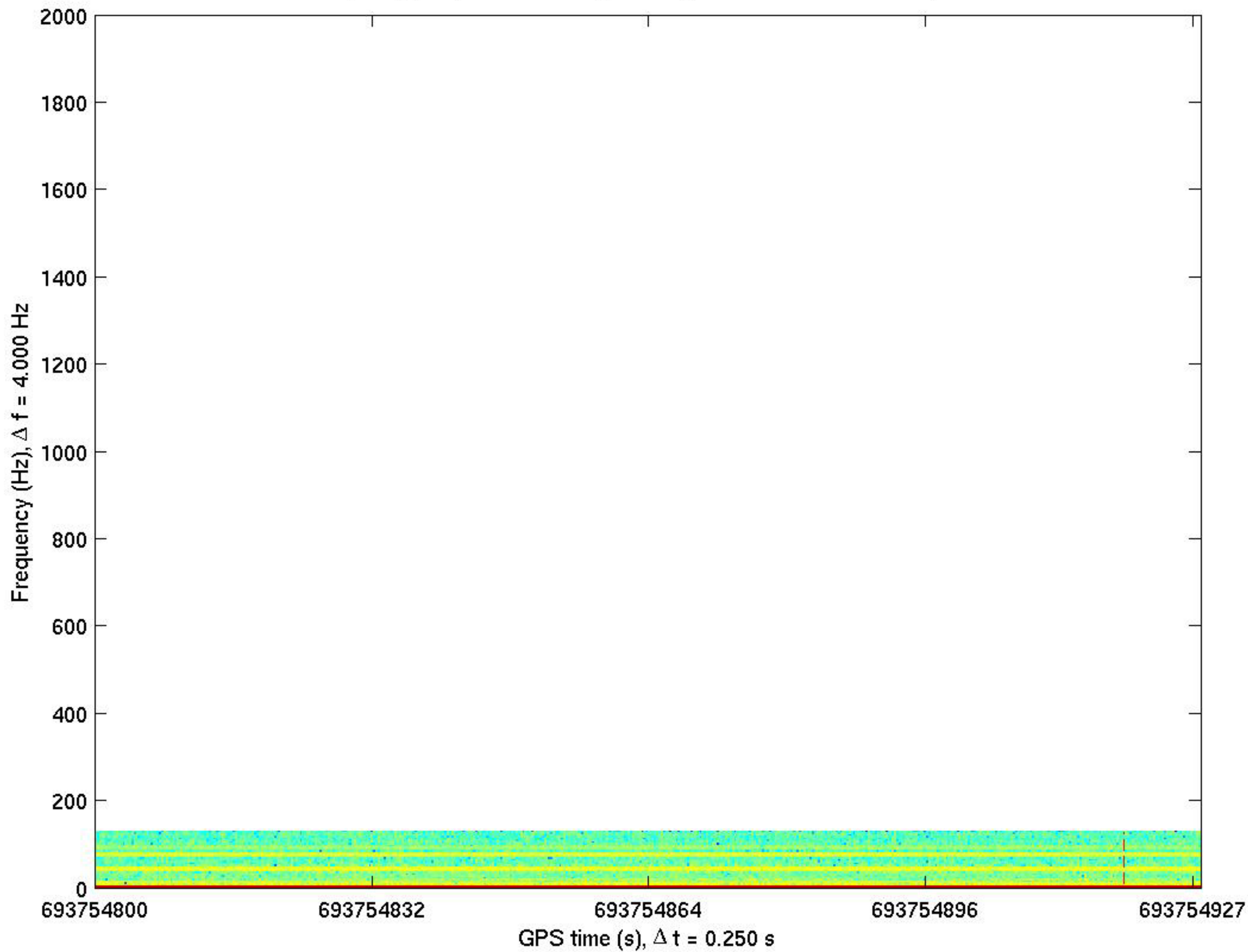
Time frequency plot, L1:PSL-FSS R FPDDC F , 693754800-693754928, T = 128 s
