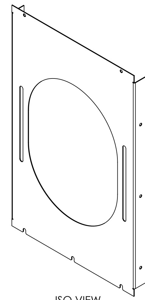
ISO VIEW
