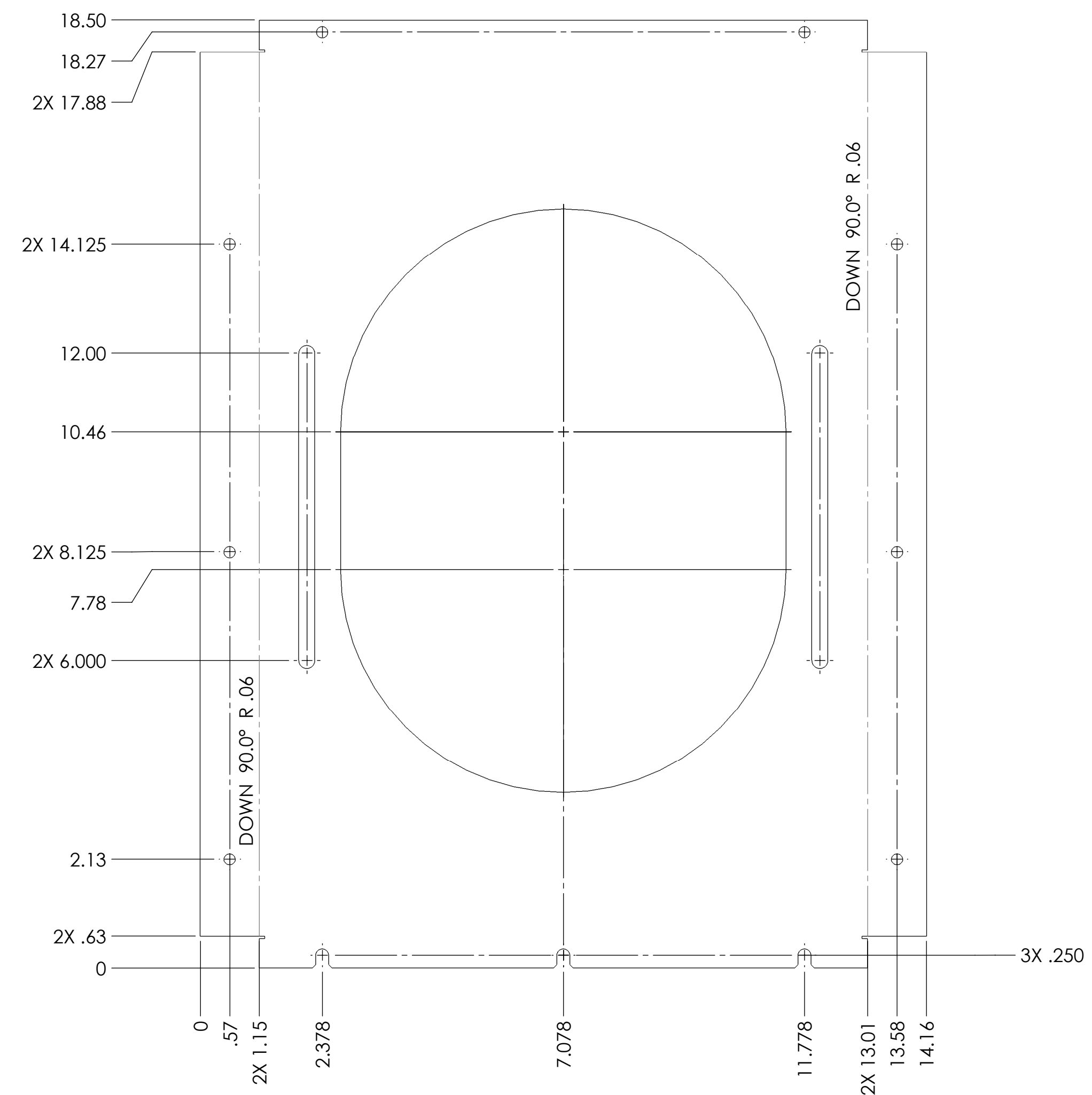
FLAT STATE (ALL DIMENSIONS SHOWN ARE FOR REFERENCE ONLY)
