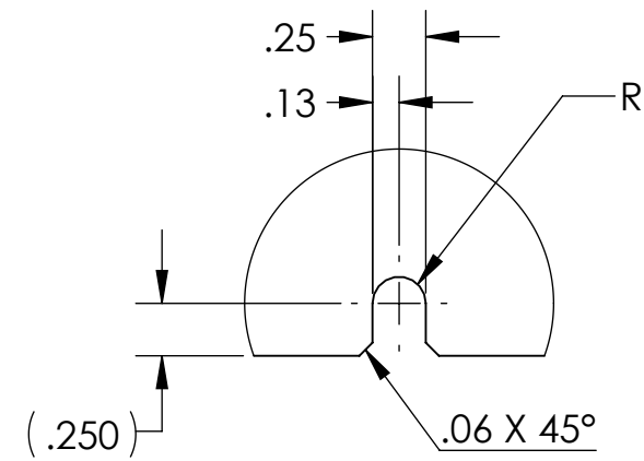
DETAIL A 3 PL. SCALE 1 : 1
