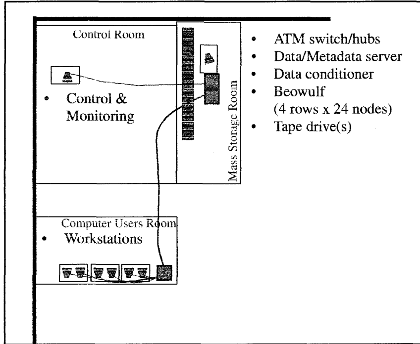
Figure 15 Layout of LDAS components within OSB rooms
