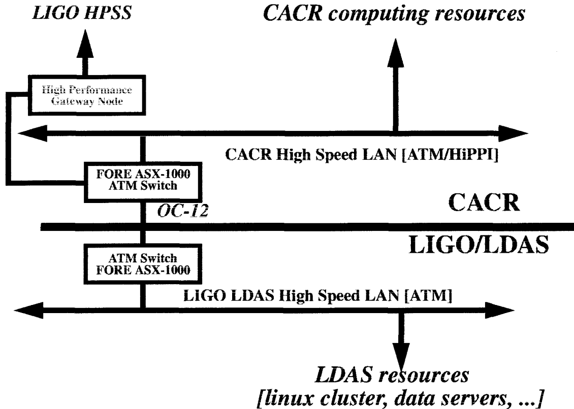
Figure 10 LDAS Networking Interfaces to CACR at Caltech
