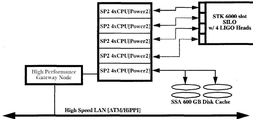
Figure 14 HPSS Configuration for LIGO
