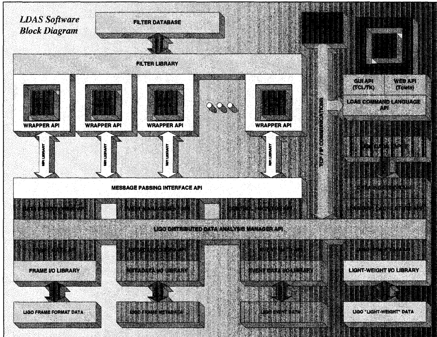
LIGO-T990001-06 Figure 4 LDAS Software Design
