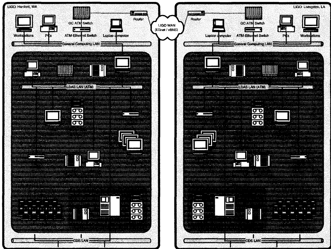
Figure 2 LDAS On-Line Configuration Overview
