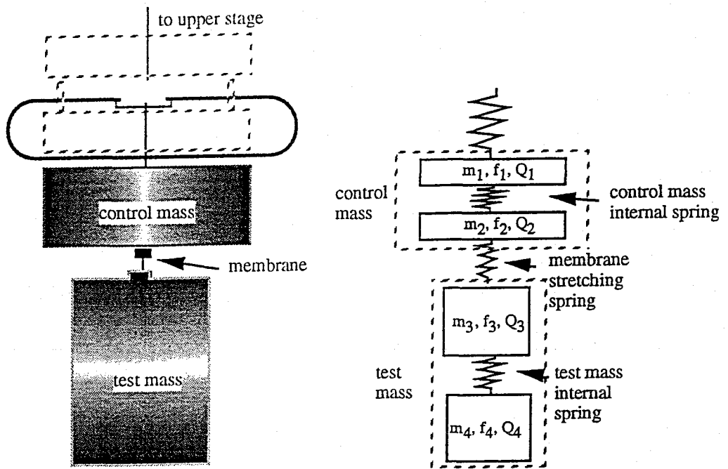
Fig 3. Model one: test mass suspended directly under control mass. A four stage spring mass model is used. Spring 1 -- spring of the whole isolator; spring 2 -- internal spring of the control mass; spring 3 -- test mass membrane flexure stretching spring; spring 4 -- equivalent test mass internal spring
