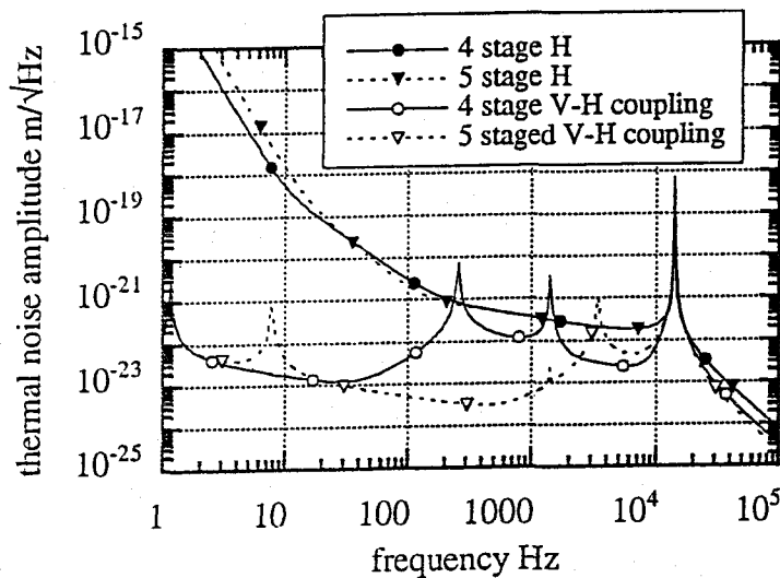
Fig. 8 Horizontal thermal noises of the systems shown in figures 3 & 4. The vertical to horizontal coupling is obtained by determining the differential thermal noise across the test mass internal spring (see figure 3 & 4), corrected by the Poisson ratio of the test mass (0.29).
