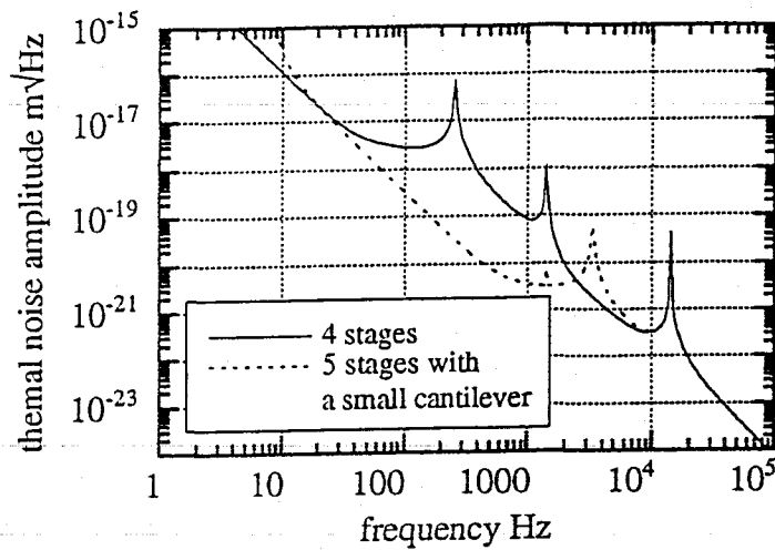
Fig. 7 Vertical thermal noise of the system shown in figures 3 & 4. The amplitudes of the resonances are not accurate because of the plot points problem.
