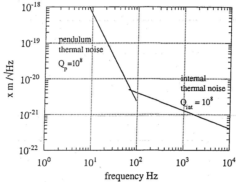
Fig.1 Predicted thermal noise of a sapphire test mass. The intrinsic Q -factor of the test mass is chosen as 10^8 . The pendulum Q factor is chosen as 10^8 with a niobium membrane flexure Q -factor of 10^5 .
