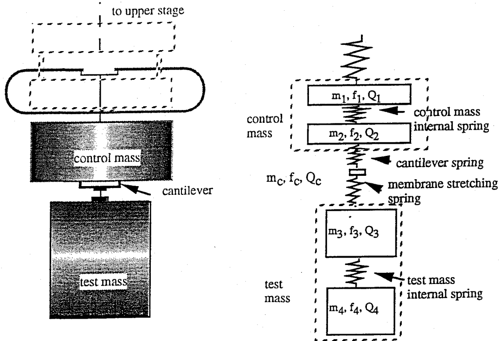
Fig. 4 Model 2: test mass suspended under a low loss, low mass cantilever which in turn is connected to the control mass. A five stage spring and mass model is used. Spring C --cantilever spring; the other elements are the same as in model 1 (figure 3).
