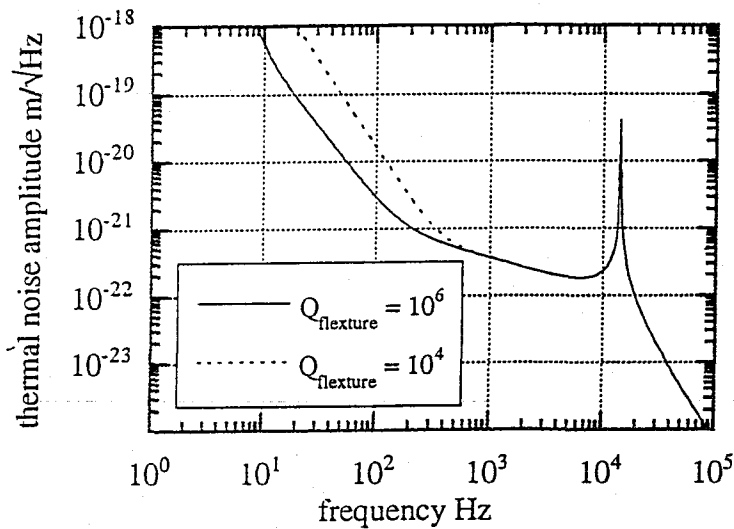
Fig. 9 Comparison of the thermal noise of membrane suspended sapphire test mass with different membrane flexure Q -factors.
