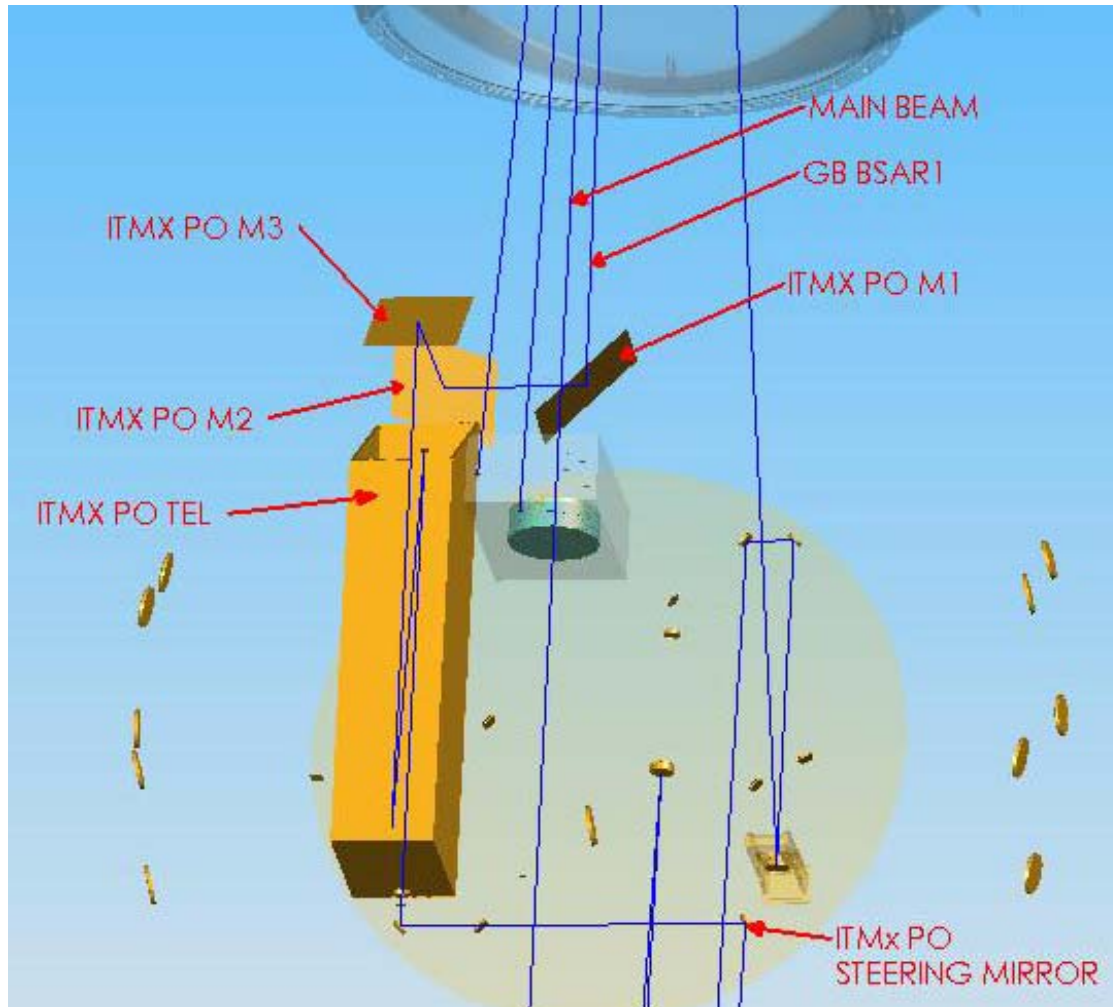
Figure 5: ITMx PO Telescope optical train
