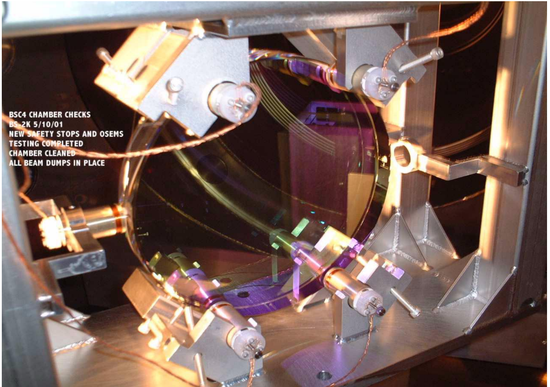
BSC4 BS as viewed from AR surface (back side), looking NE.
