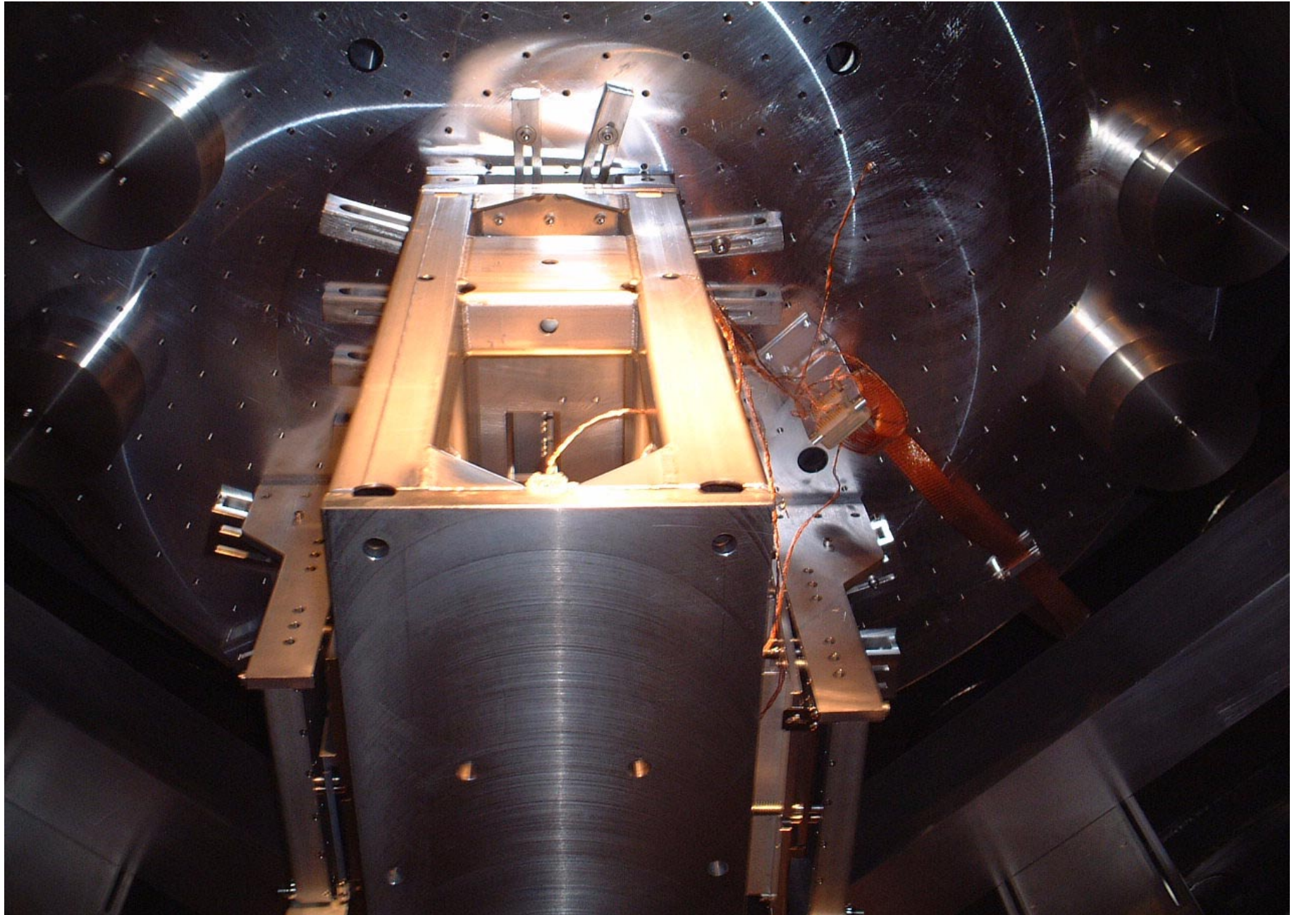
BSC4 BS Suspension tower as viewed from below. ITMy Pick Off mirror is to the right of the tower. ITMx Pick Off mirror is to the left. The PSL input beam comes in from the left side of the tower.
