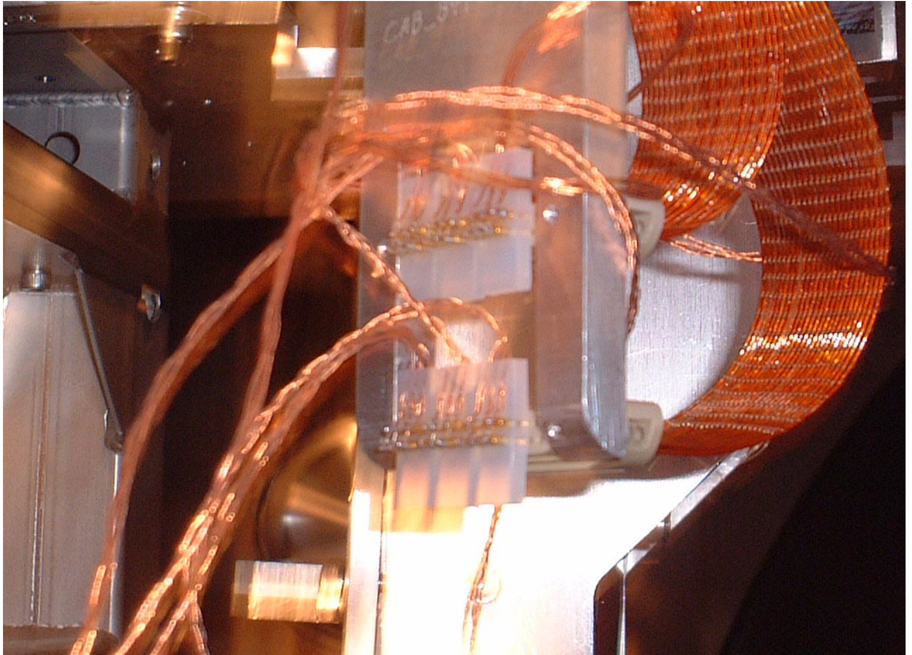
BSC 4 2k BS Sensor/Actuator cable connections.
