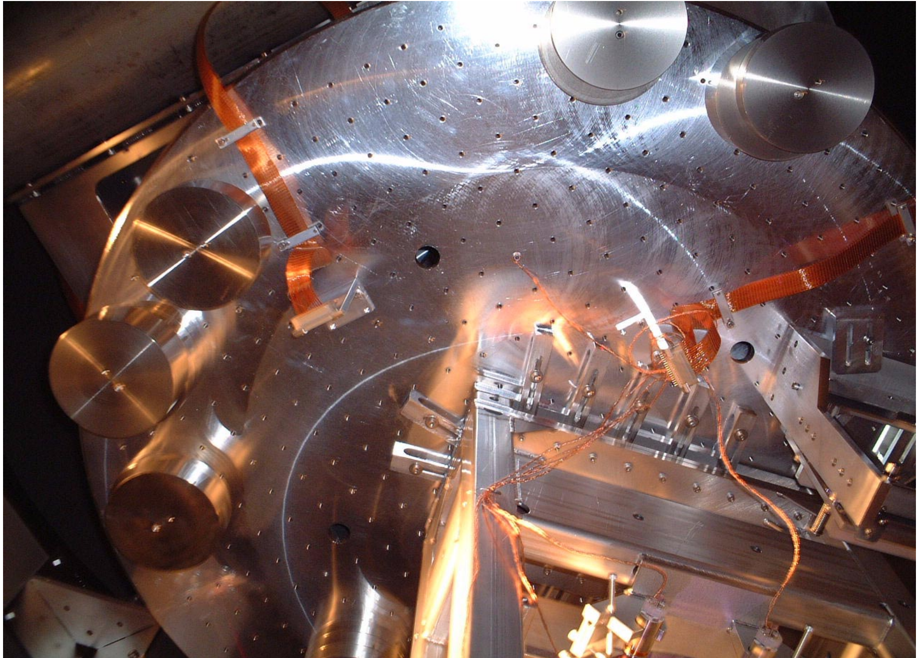
BSC4 BS Tower as viewed from below the optics table. ITMy Pick Off mirror is to the right of the tower.
