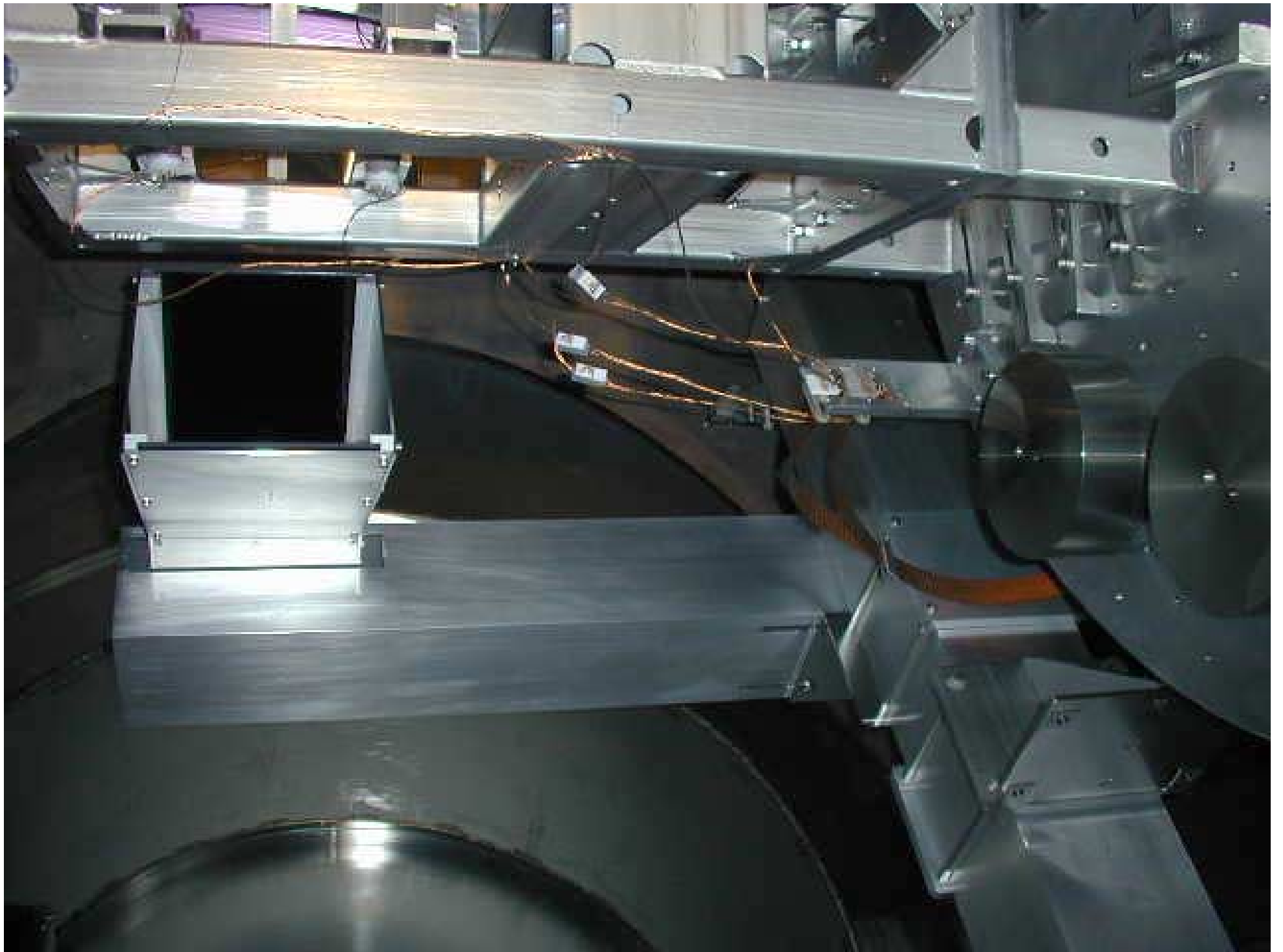
WBSC 8 May 12, 2000: 009. Beam dump @ E port
