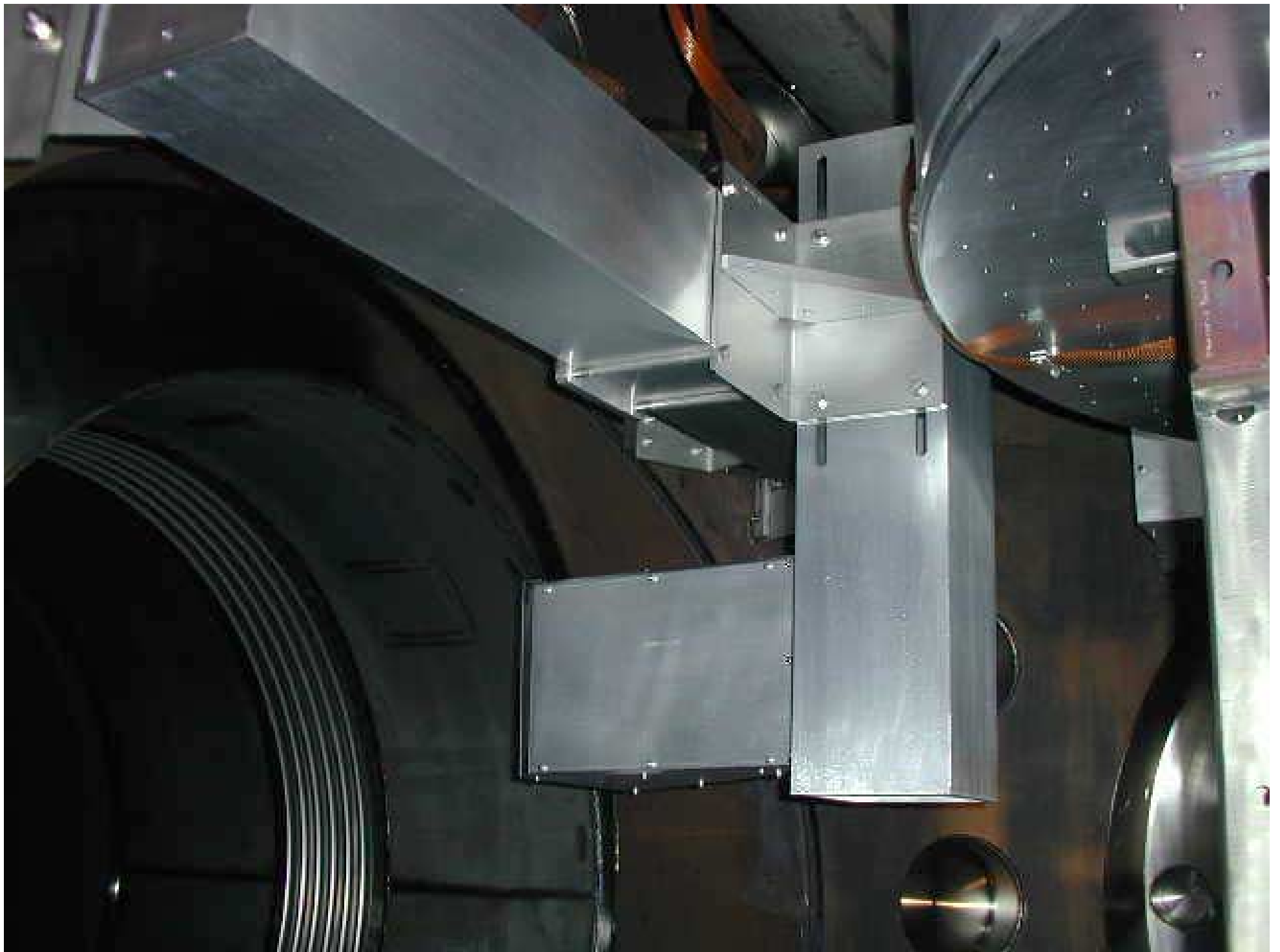
WBSO 8 May 12, 2000: 007. Beam dump @ N port
