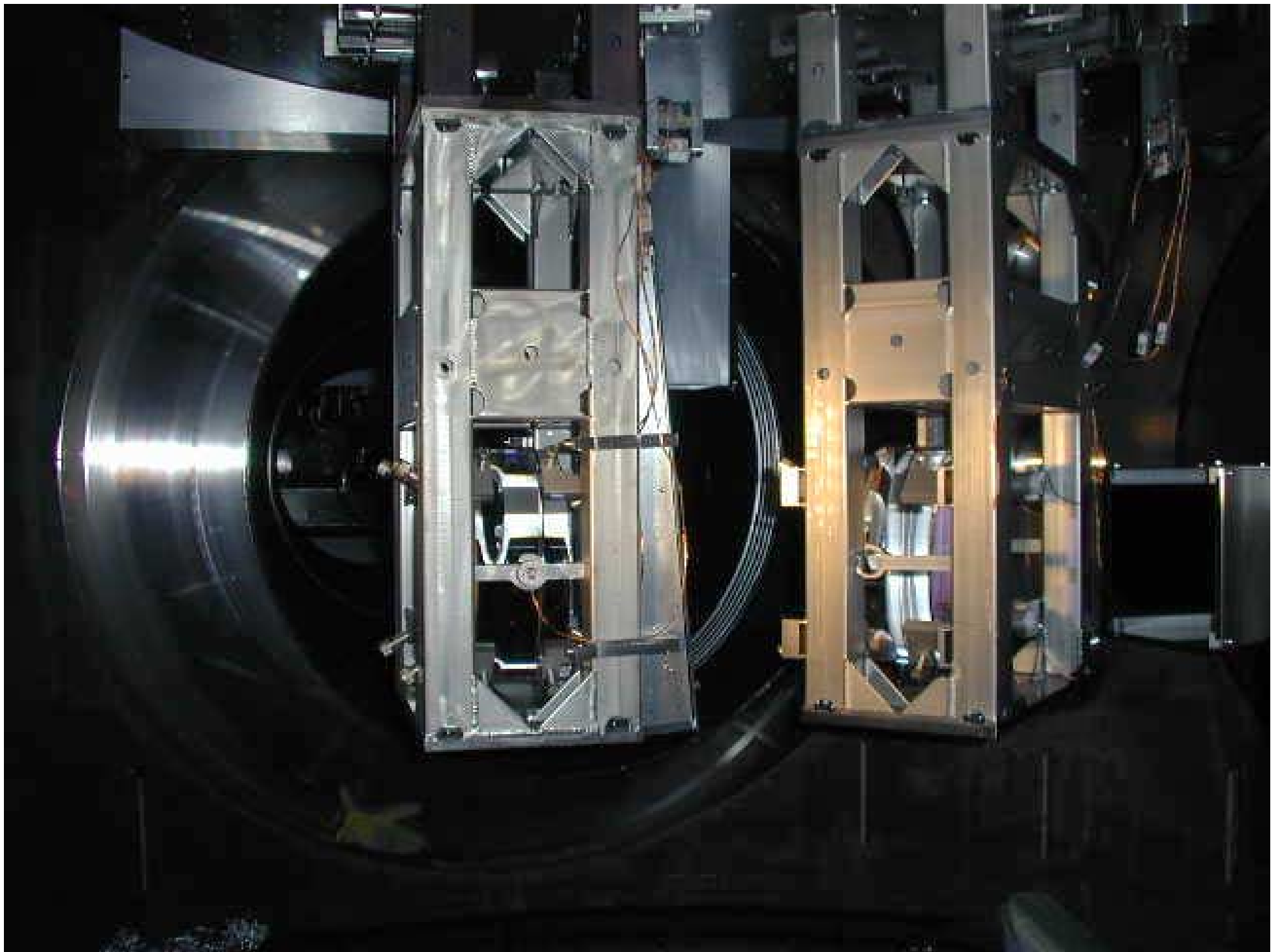
WBSC 8 May 12, 2000: 010. ITMy, Fmy
