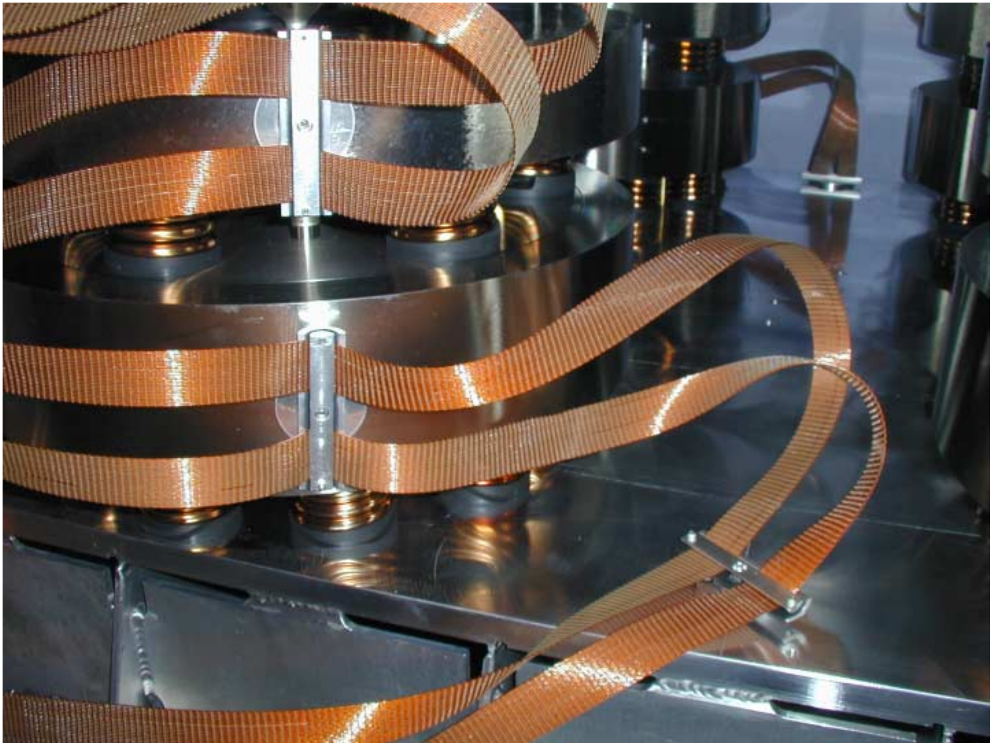
WHAM 7 May 18, 2000: 018. NW stack, from W (post tune)
