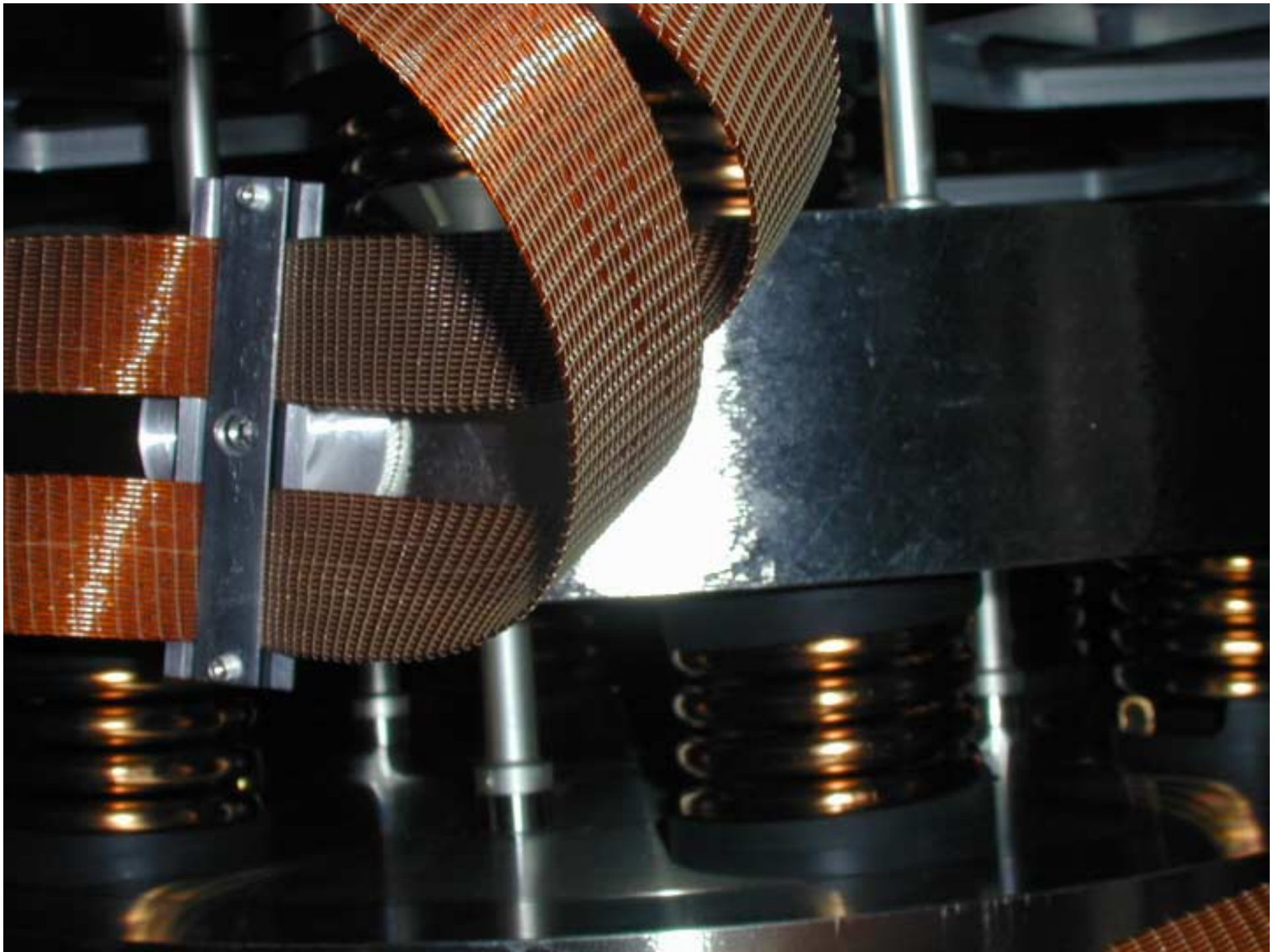
WHAM 7 May 18, 2000: 017. NW stack, from W (cables touching, mid photo)
