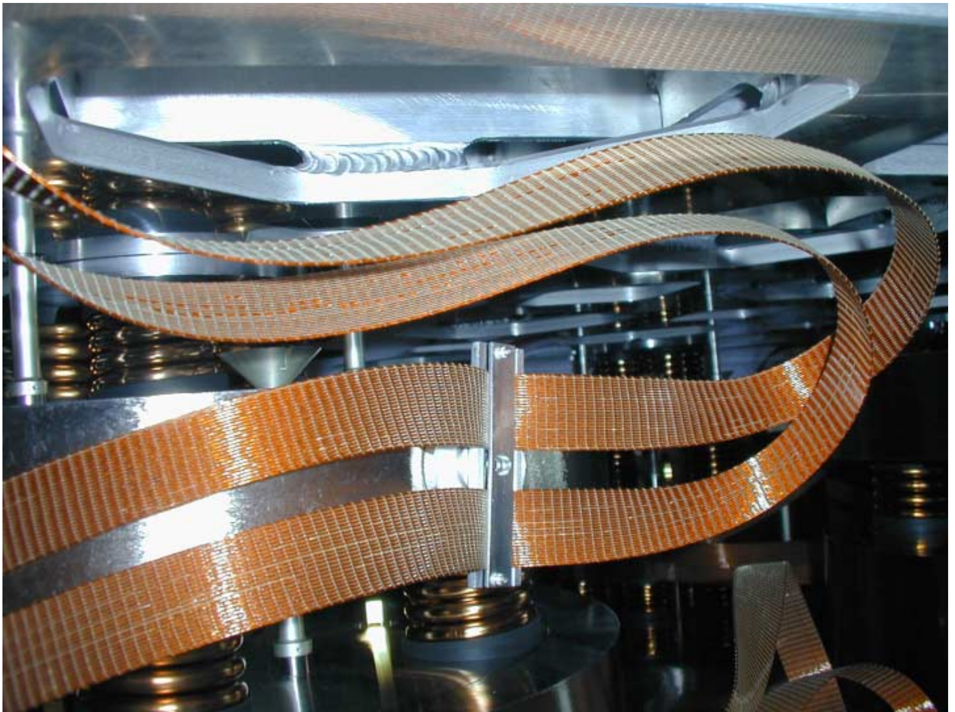
WHAM 7 May 18, 2000: 016. NW stack, from W (cables touching @ right)
