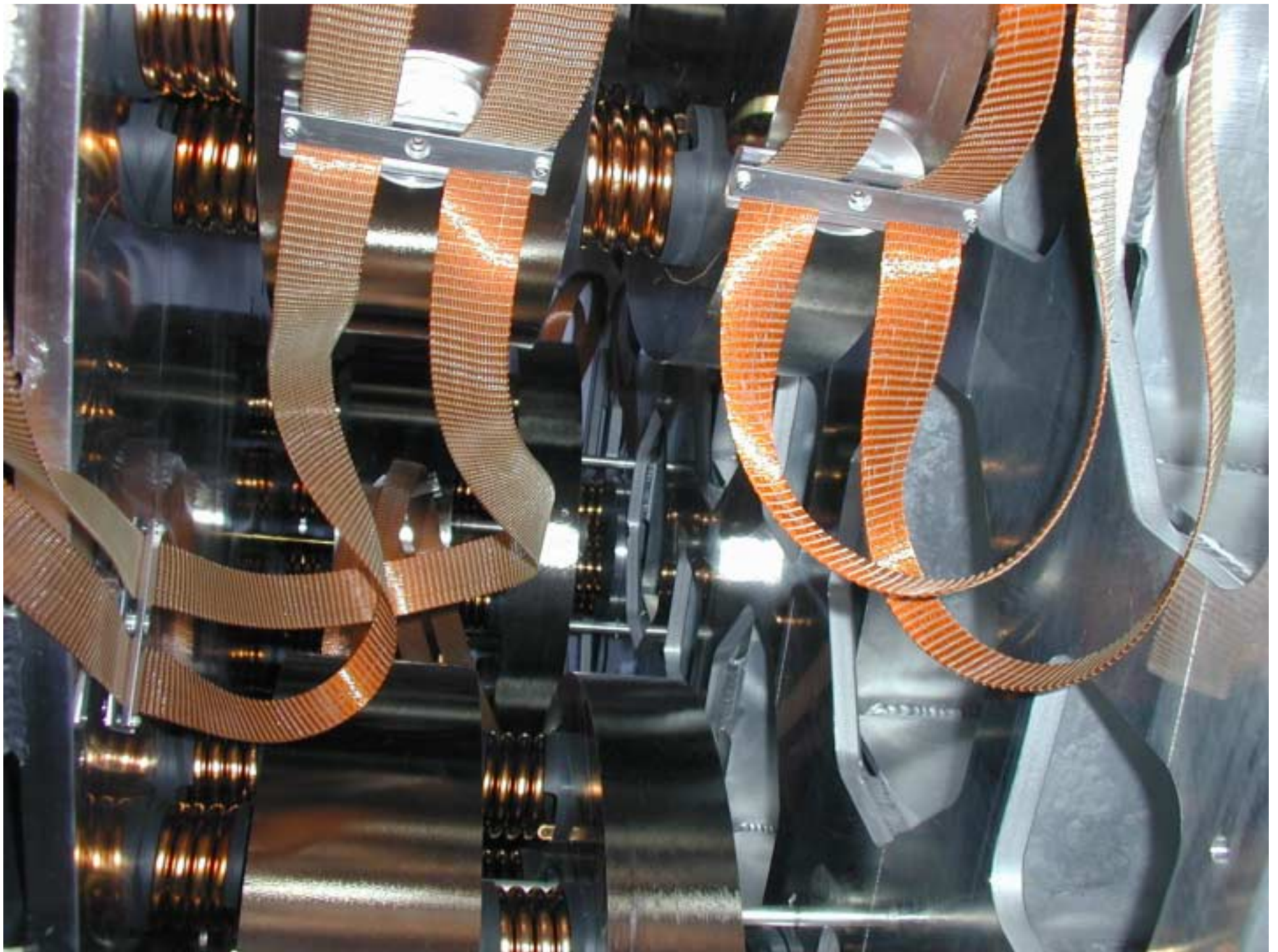
WHAM 7 May 18, 2000: 021. NW stack, from W (post tune)
