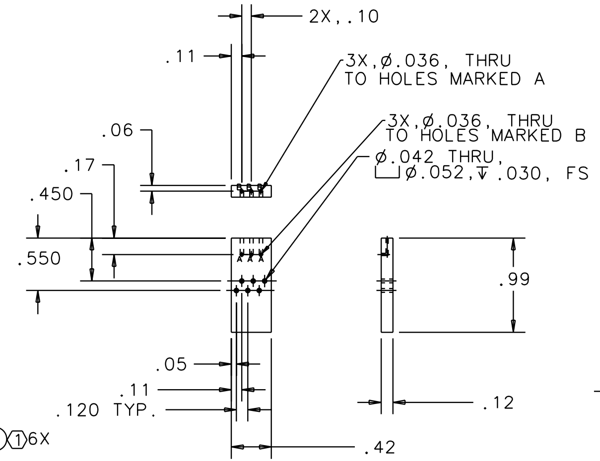
PIGTAIL RECTANGULAR PLATE DETAIL, ITEM 2 SCALE: 1/1
