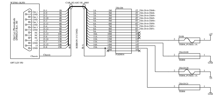
WA2K FM1 Opt Lever PD
