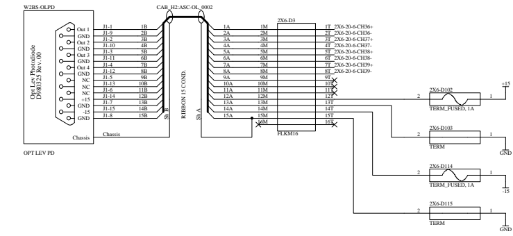
WA2K BS Opt Lever PD
