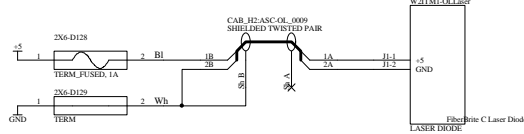
WA2K ITM1 Opt Lever Laser Diode
