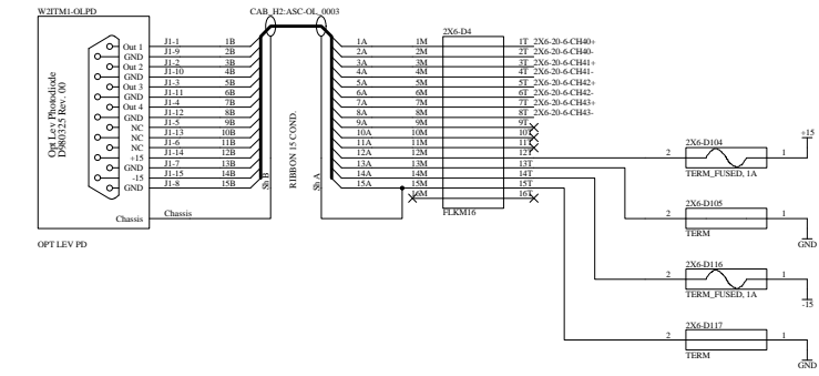
WA2K ITM1 Opt Lever PD
