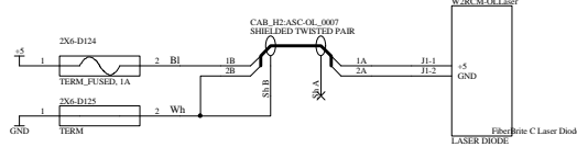
WA2K RCM Opt Lever Laser Diode
