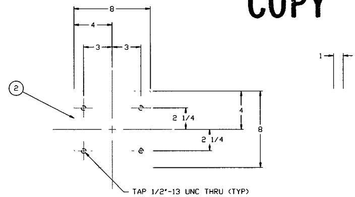
DETAIL '3' QTY: 4
