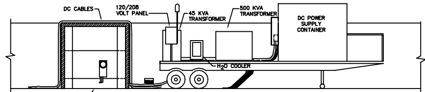
FRONT VIEW TYPICAL DC POWER SUPPLY PORT - EQPT. ARRANGEMENT
