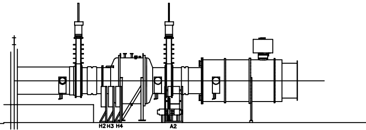
ELEVATION TYPICAL CORNER/MID/END STATION POWER EQPT.
