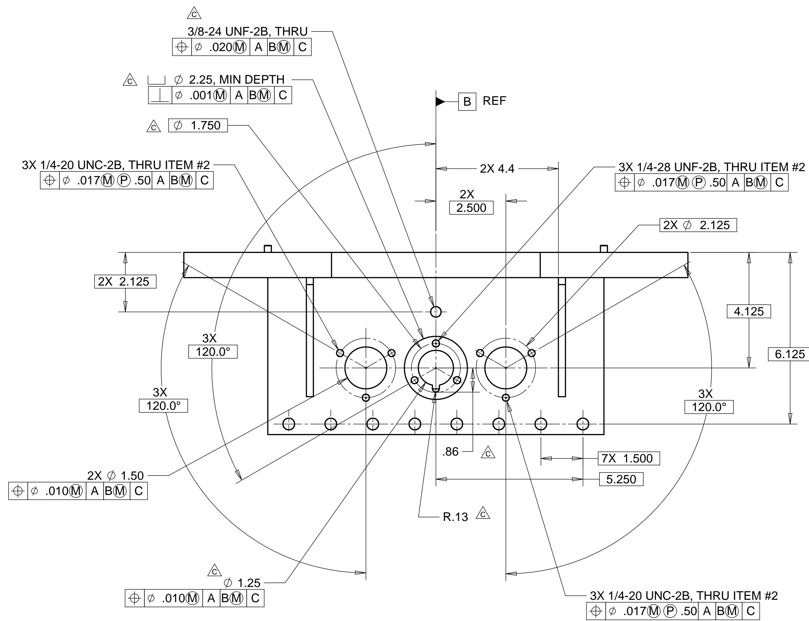
VIEW B - B FROM SHEET 1
