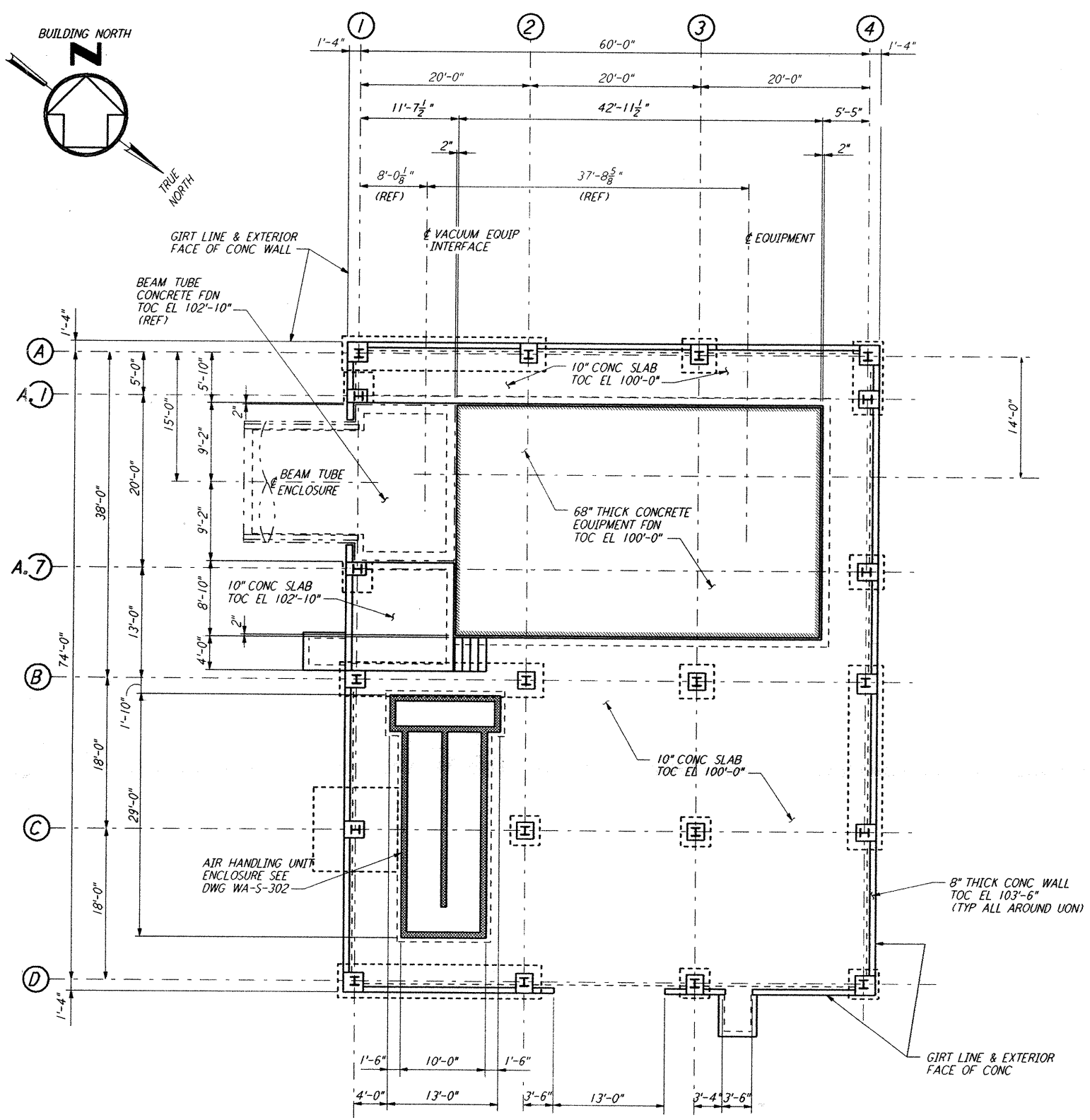
END STATION FOUNDATION PLAN 1/8" = 1'-0"
