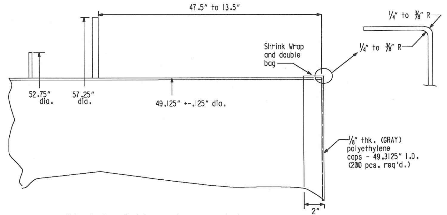
Tube Section End Covers (pre-expansion)
