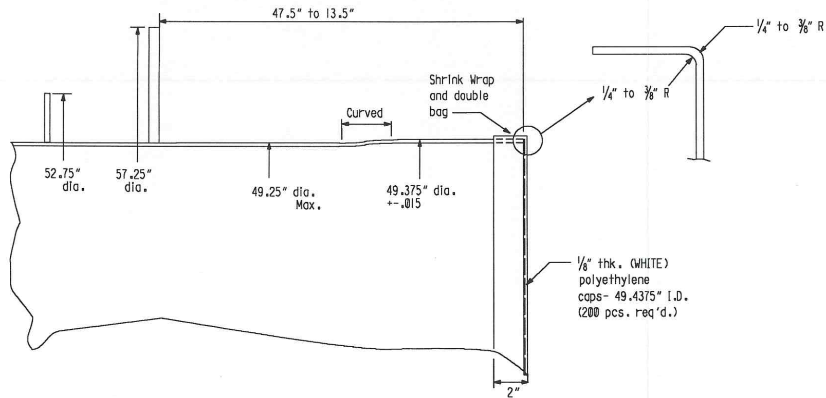
Tube Section End Covers (post-expansion)
