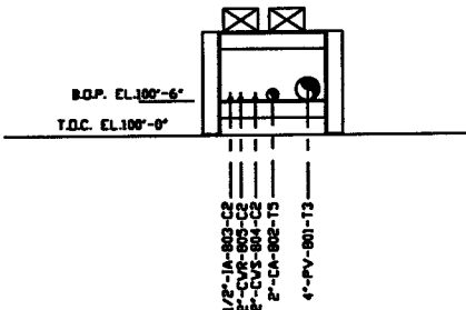
SECTION A SCALE: 3/4"=1'-0" V049-5-021, SHT1
