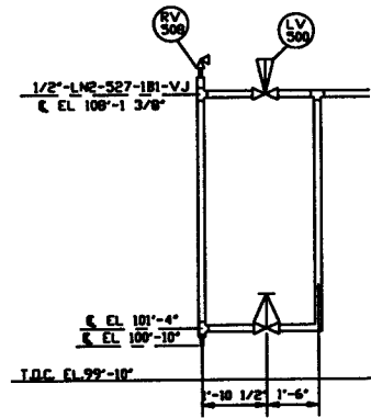
SECTION B SCALE: 3/8"=1'-0" V049-5-021, SHT2
