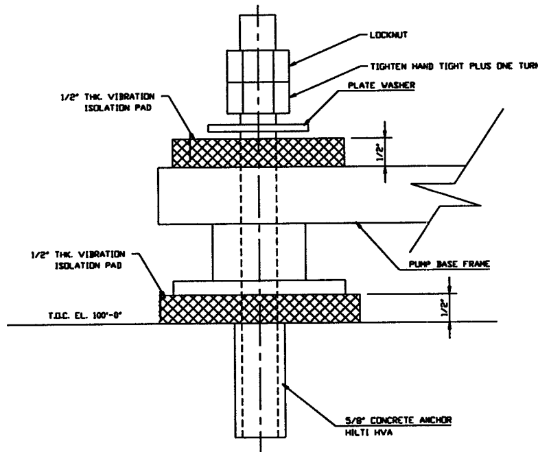
DETAIL 2 SCALE: FULL V049-5-021, SHT1
