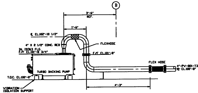
SECTION C SCALE: 3/4"=1'-0" V049-5-021, SHT1
