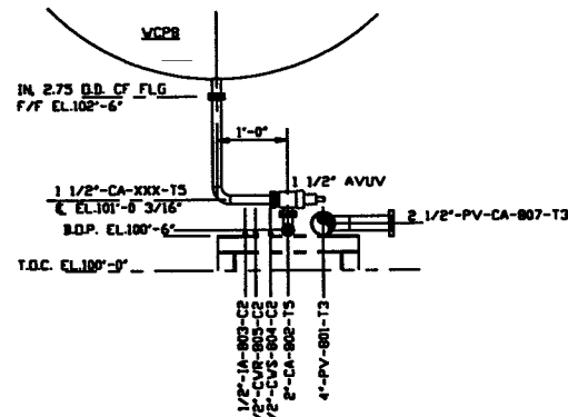
SECTION D SCALE: 3/4"=1'-0" V049-5-021, SHT1
