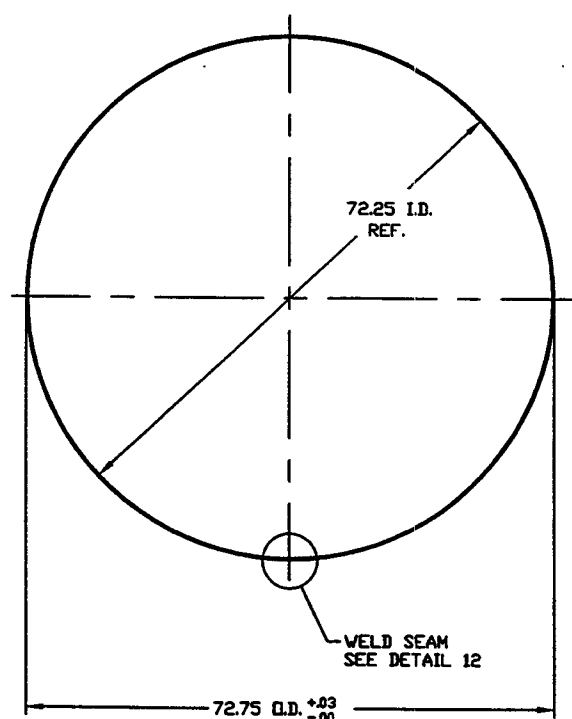
DETAIL "15" QTY: 1 MAKE FROM V049M154-1
