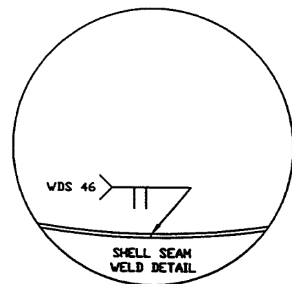
DETAIL "12" SHELL SEAM PREP & WELD
