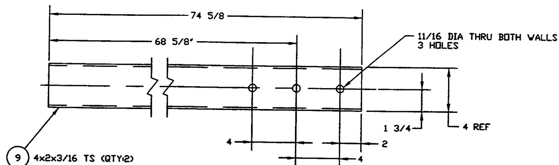
DETAIL "1"
