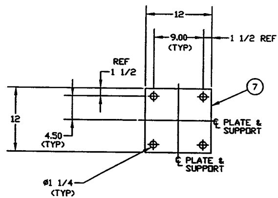
DETAIL "17" QTY: 2
