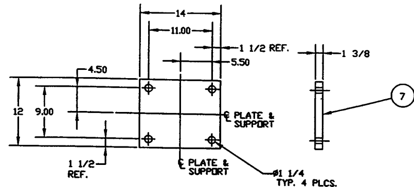
DETAIL "8" QTY: 2
