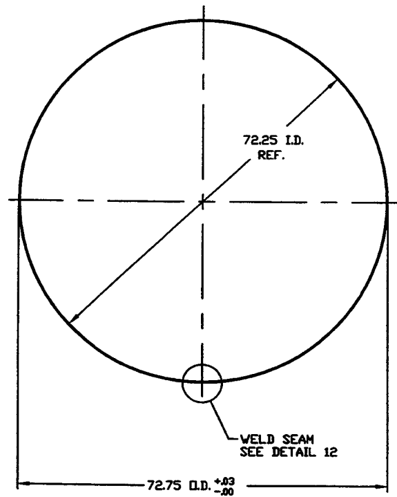
DETAIL "3" QTY: 3 MAKE FROM V049M154-1
