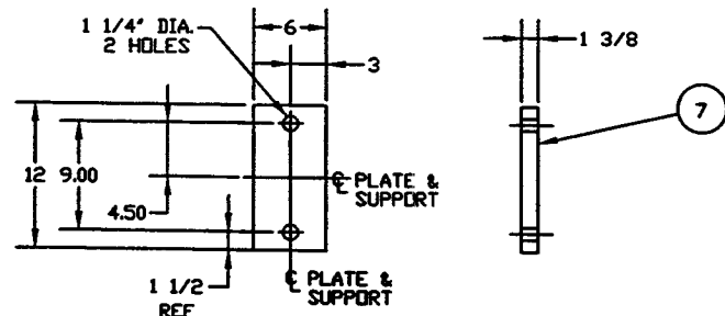
DETAIL "2" QTY: 2
