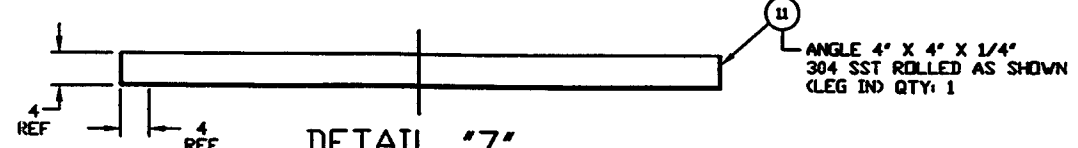
DETAIL "7"
