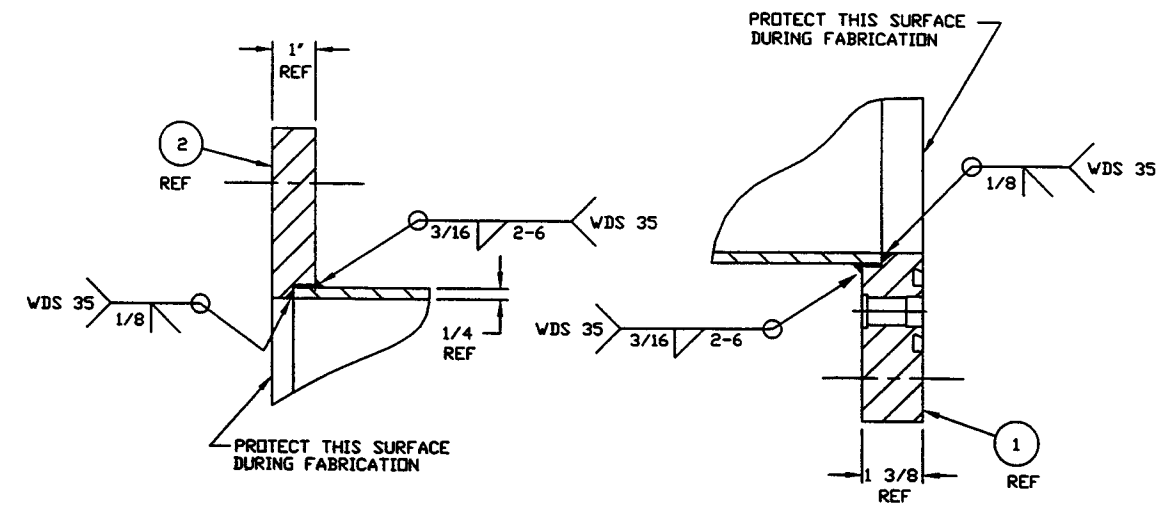
DETAIL "5"
