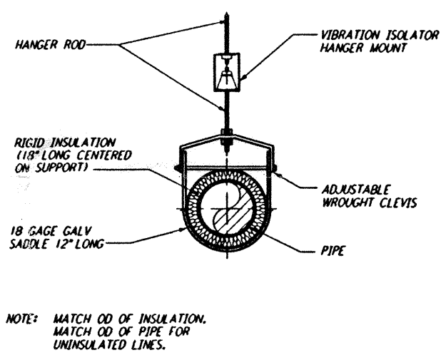
PIPE HANGER DETAIL - SINGLE PIPE 6 REF NTS LA-P-411
