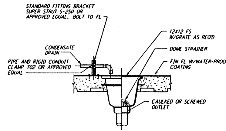
FLOOR SINK DETAIL 3 REF NTS LA-P-411
