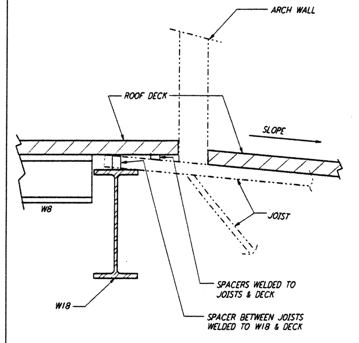
SECTION D REF NTS LA-S-407 LA-S-116
