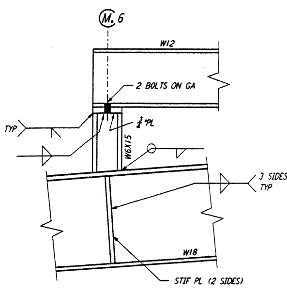
DETAIL 1 REF NTS LA-S-407 LA-S-120
