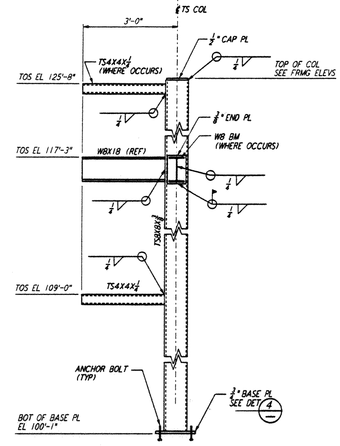
SECTION C REF NTS LA-S-407 LA-S-116 LA-S-123
