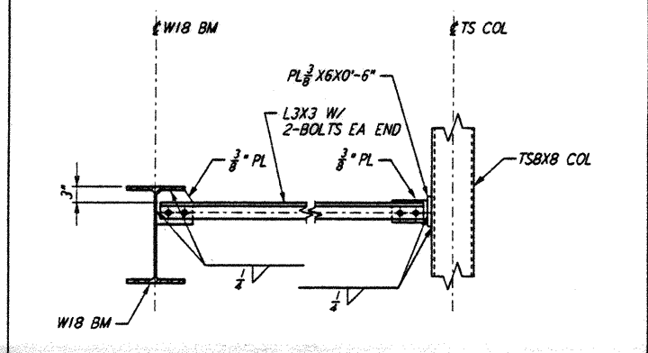
DETAIL 5 REF NTS LA-S-407 LA-S-116
