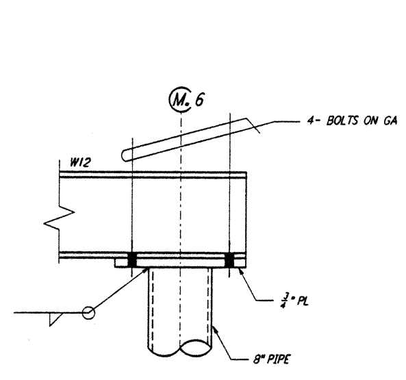
DETAIL 2 REF NTS LA-S-407 LA-S-119 LA-S-120
