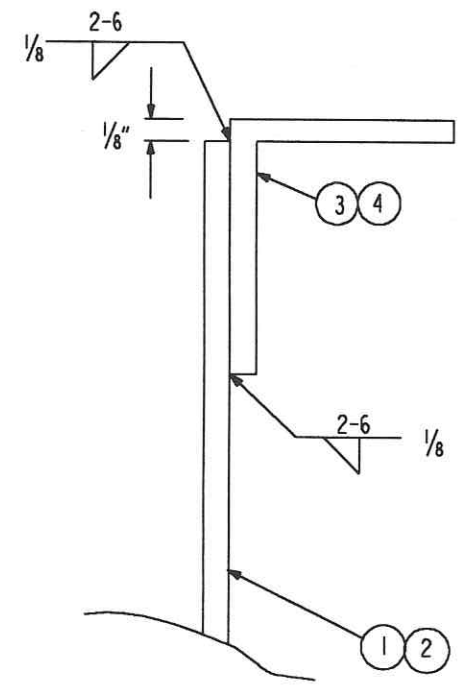
Typical angle weld detail
