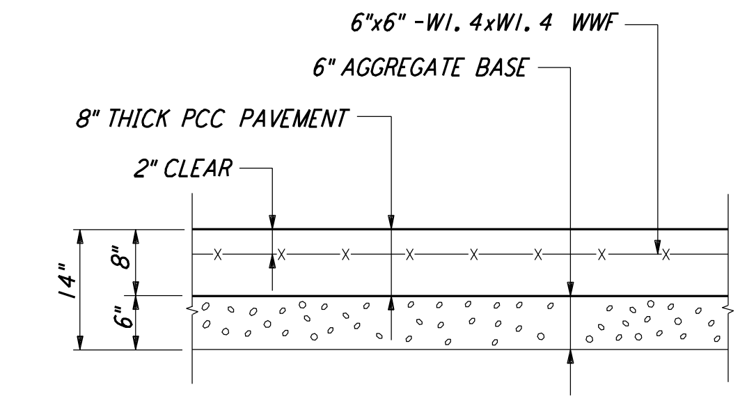
CONCRETE PAVEMENT (2) NOT TO SCALE REF: BT-C-051, BT-C-041, BT-C-045
