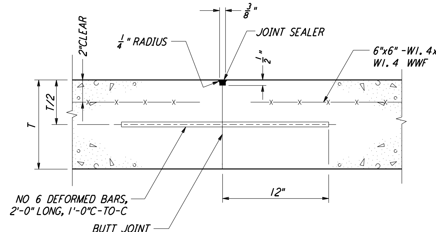
CONSTRUCTION JOINT (4) NOT TO SCALE REF: BT-C-051, BT-C-041, BT-C-045 (SEPARATE POURS OR END OF DAY)
