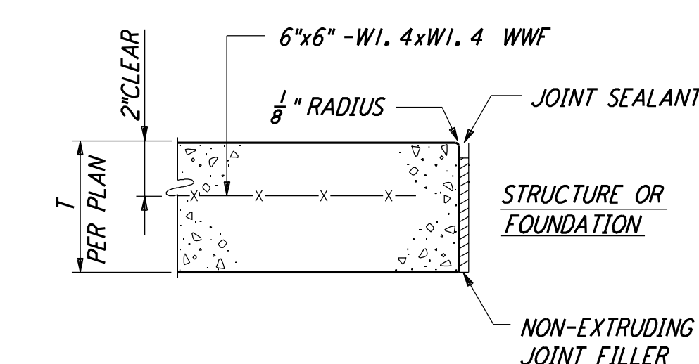
EXPANSION JOINT (3) NOT TO SCALE REF: BT-C-051, BT-C-041, BT-C-045
