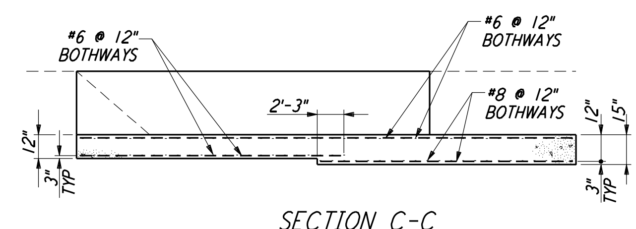
SECTION C-C
