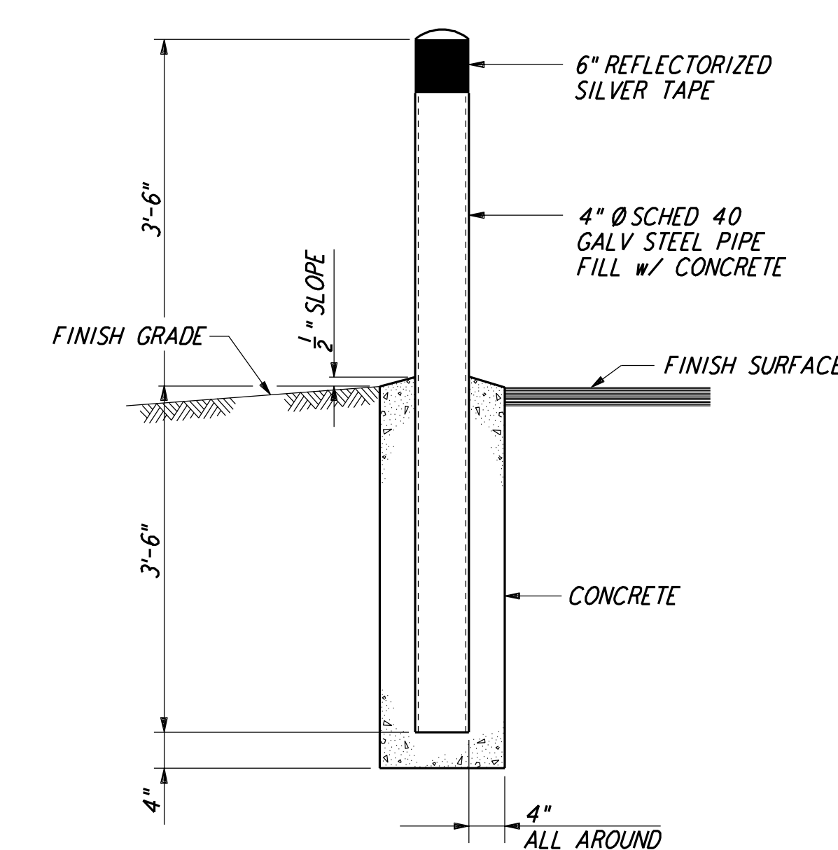
GUARD POST (7) NOT TO SCALE REF: BT-C-051, BT-C-004
