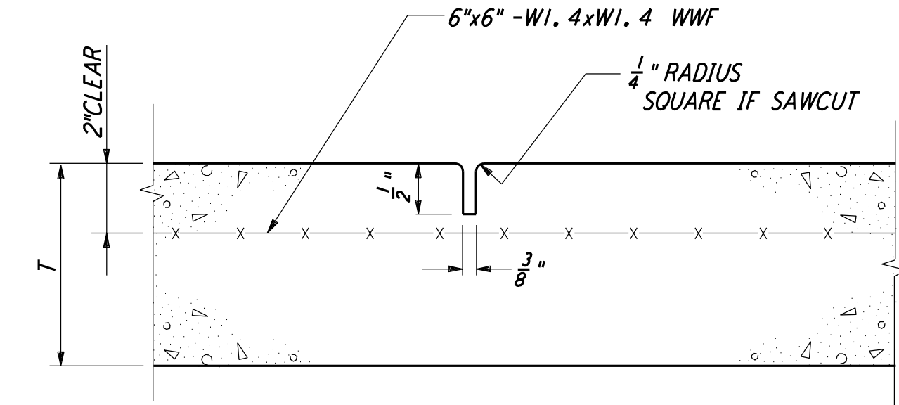
CONTRACTION JOINT (5) NOT TO SCALE REF: BT-C-051, BT-C-041, BT-C-045 (SPACING: 20' MAX)
