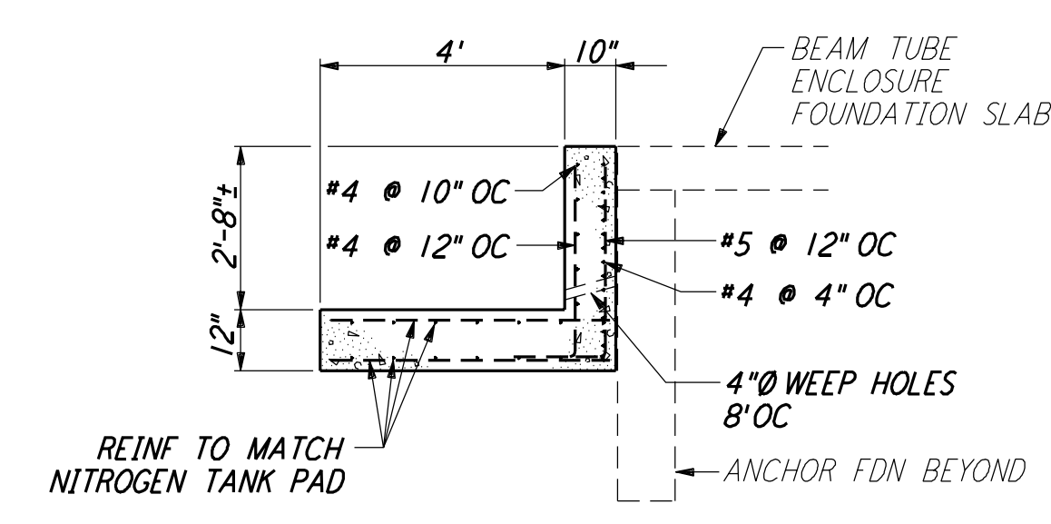
SECTION E-E
