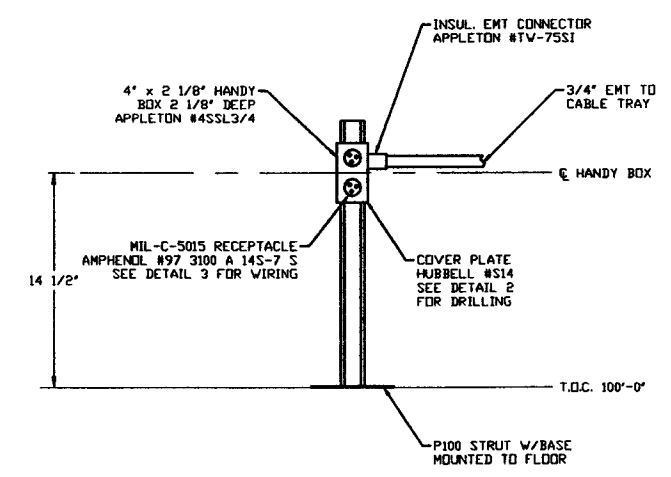
DETAIL 1 DATA HIGHWAY CONNECTION BOX MOUNTING NOSCALE
