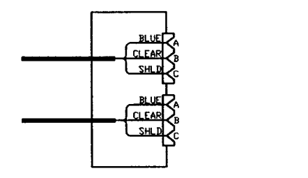
DETAIL 3 CONNECTOR WIRING OMIT WIRING FOR SECOND CONNECTOR FOR END CONNECTION BOXES NO SCALE
