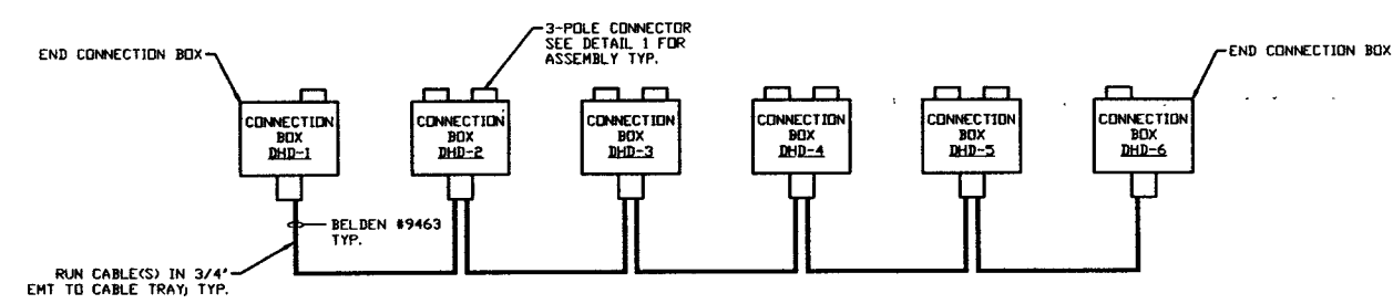
DIAGONAL SECTION DATA HIGHWAY INTERCONNECTION SEE PLAN FOR LOCATIONS
