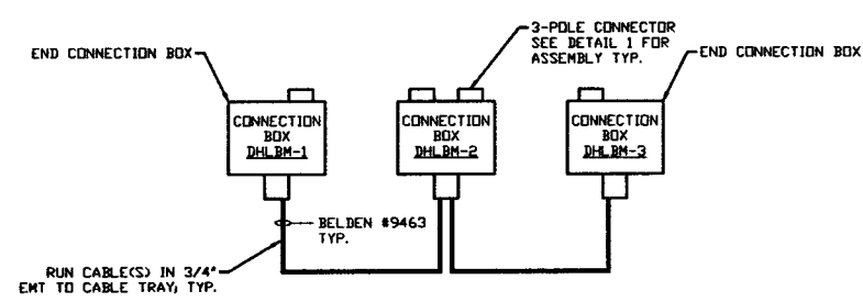
LEFT BEAM MANIFOLD DATA HIGHWAY INTERCONNECTION SEE PLAN FOR LOCATIONS
