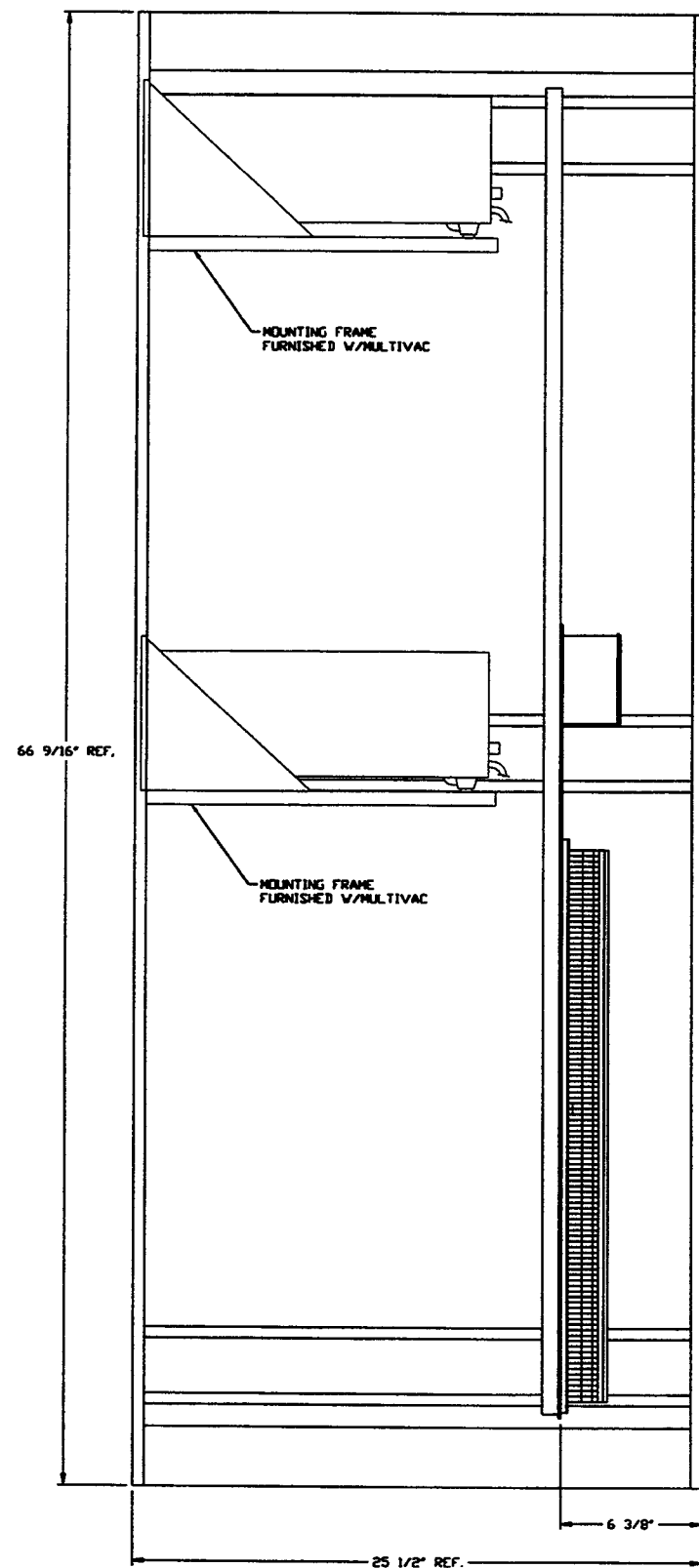
SECTION A REF. SCALE: 1/4" = 1'-0" --- V049-3-121 SHY. 1
