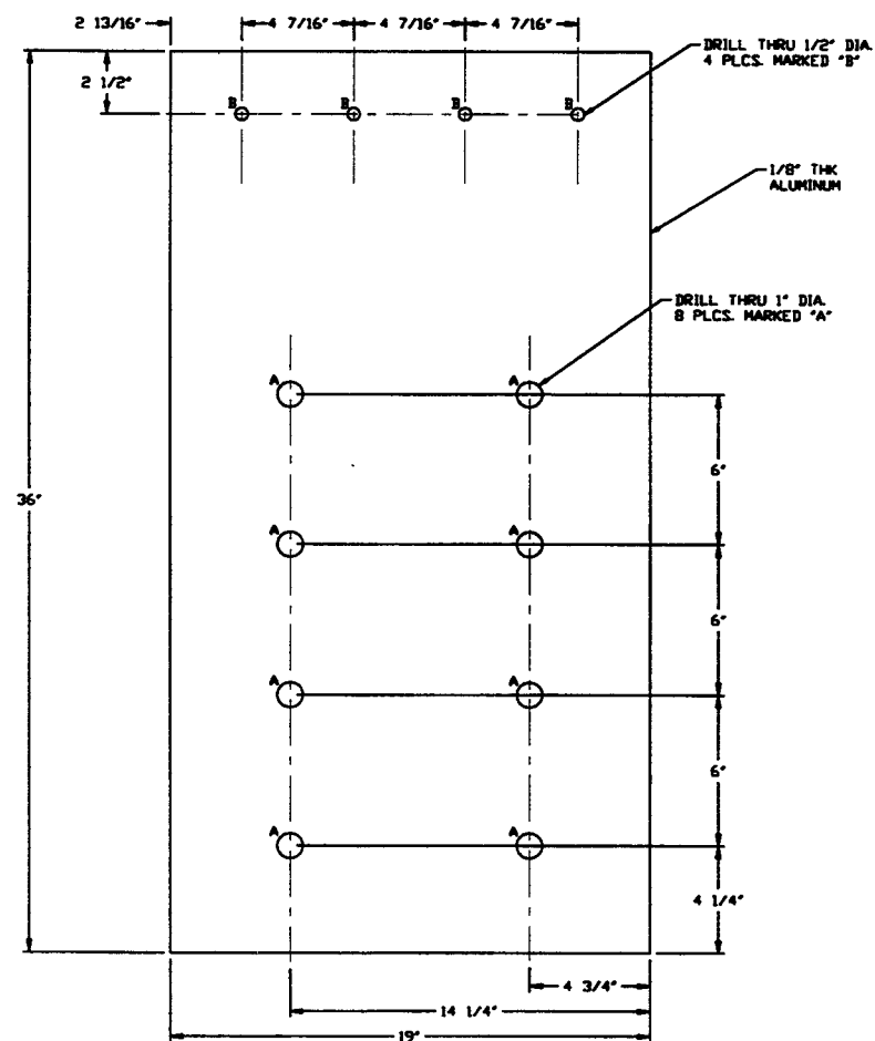
DETAIL 1 REF. SCALE: 1/4" = 1'-0" --- V049-3-121 SHY. 1
