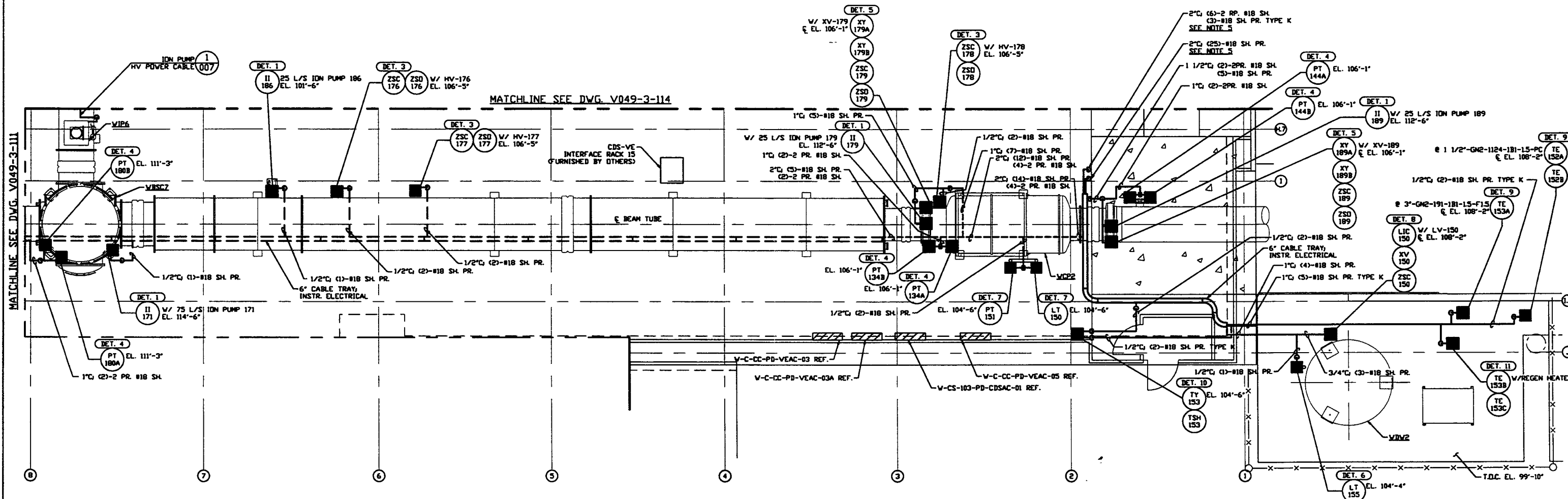
RIGHT BEAM MANIFOLD PLAN @ EL. 100'-0"
